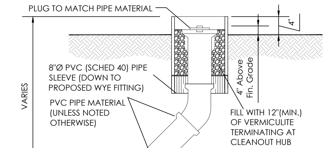
EXTERIOR CLEANOUT SECTION (@ LOCATIONS WITHIN TURF AREAS)
