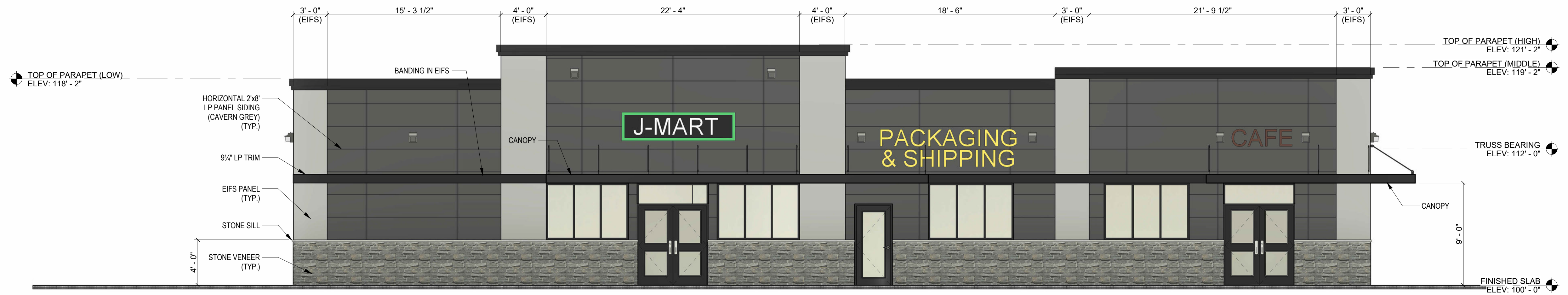
SOUTH ELEVATION
