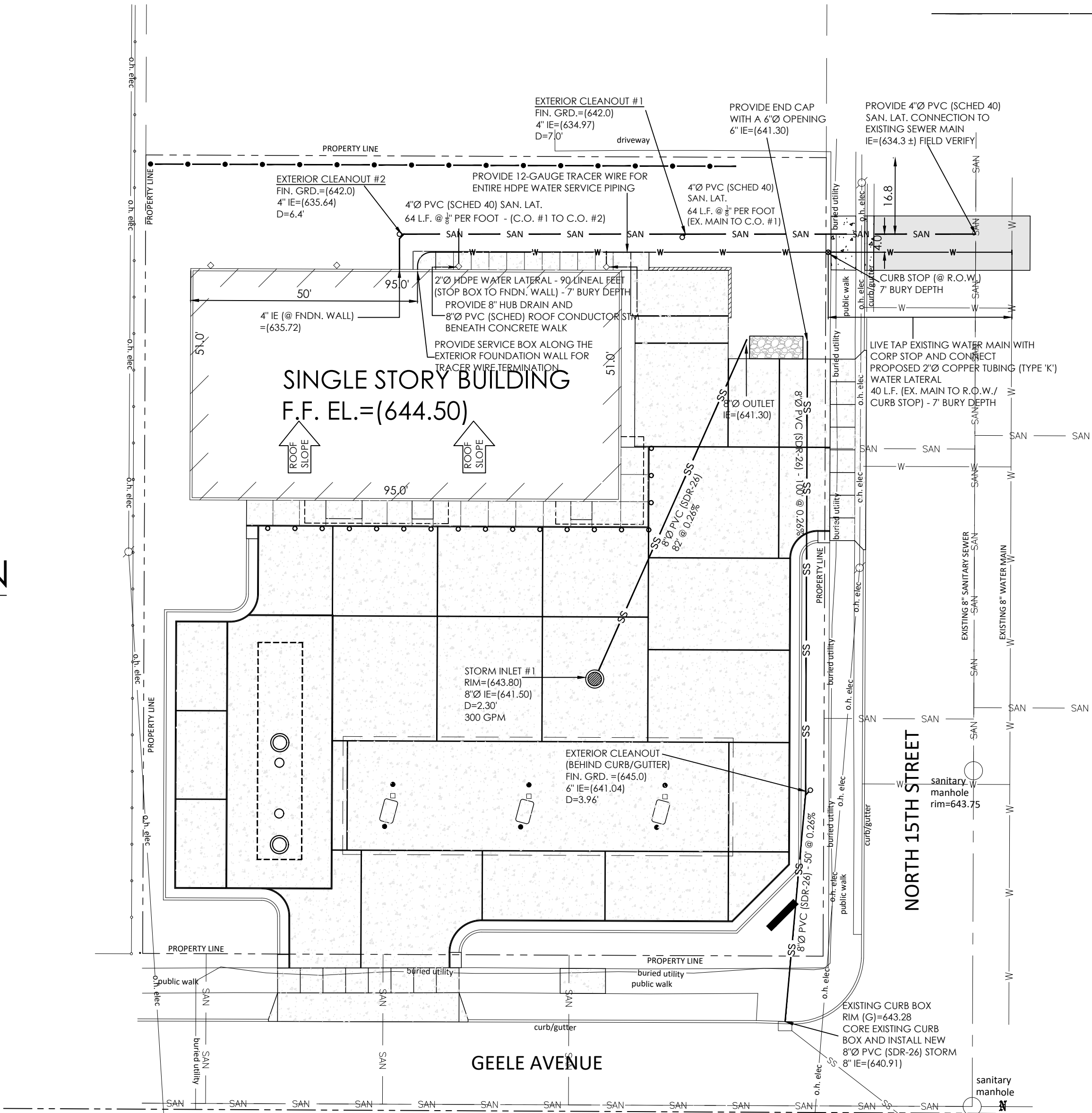
SITE UTILITY PLAN
