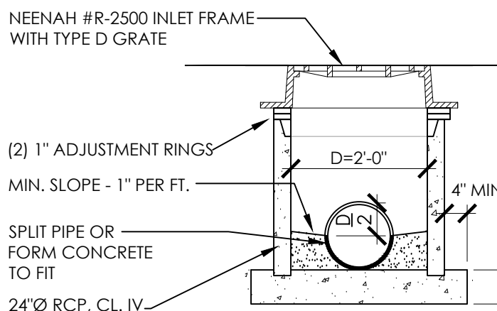
STORM INLET SECTION
