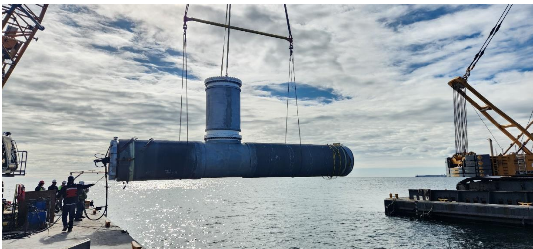
Kokosing installs emergency riser intake pipe section near sta. 50+00.
