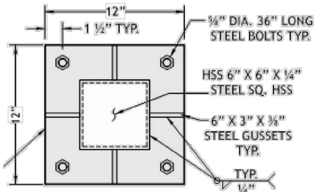
STEEL BASE PLATE
