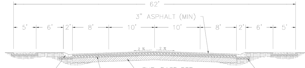
ROADWAY CROSS SECTION
