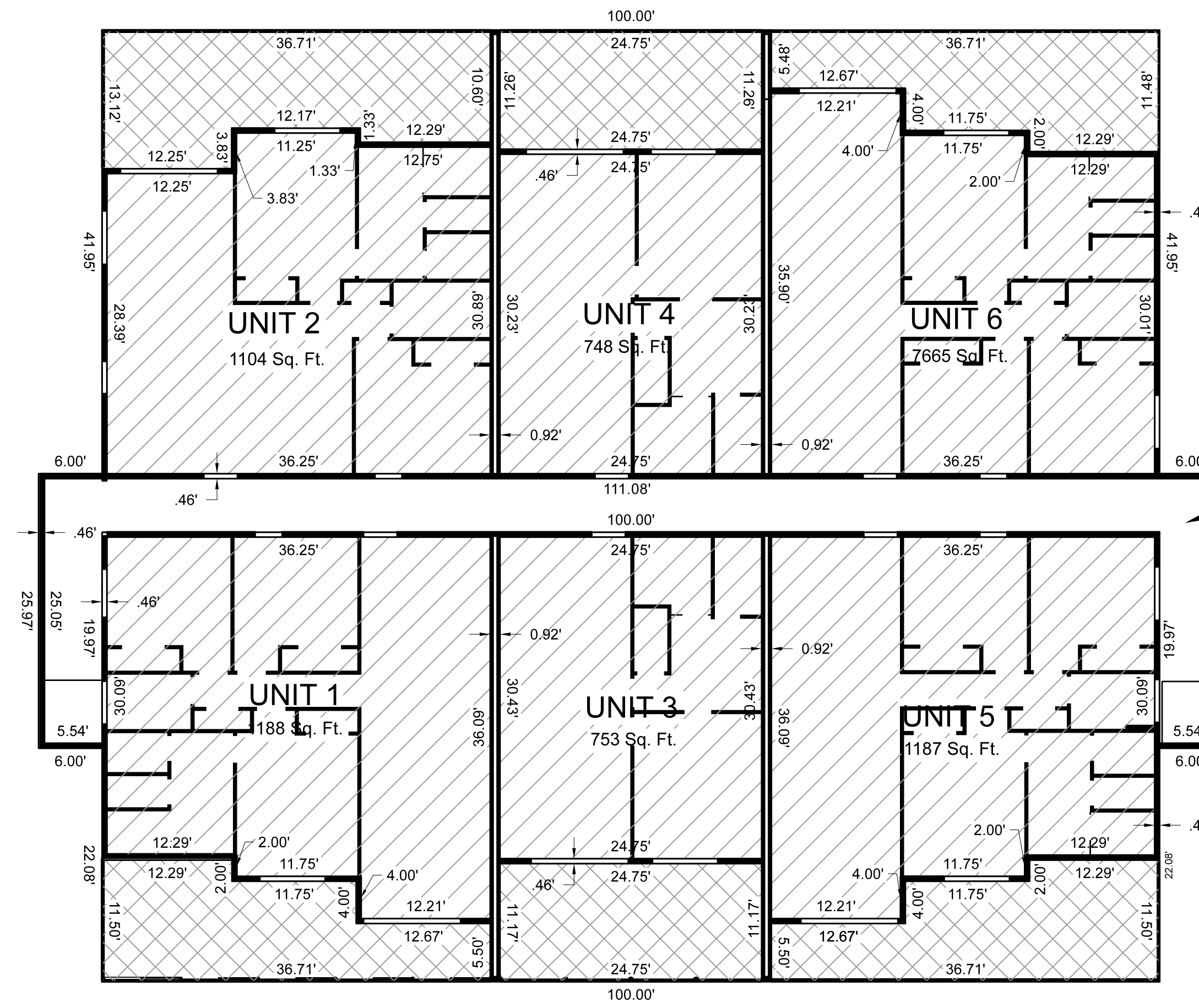
SECOND FLOOR
