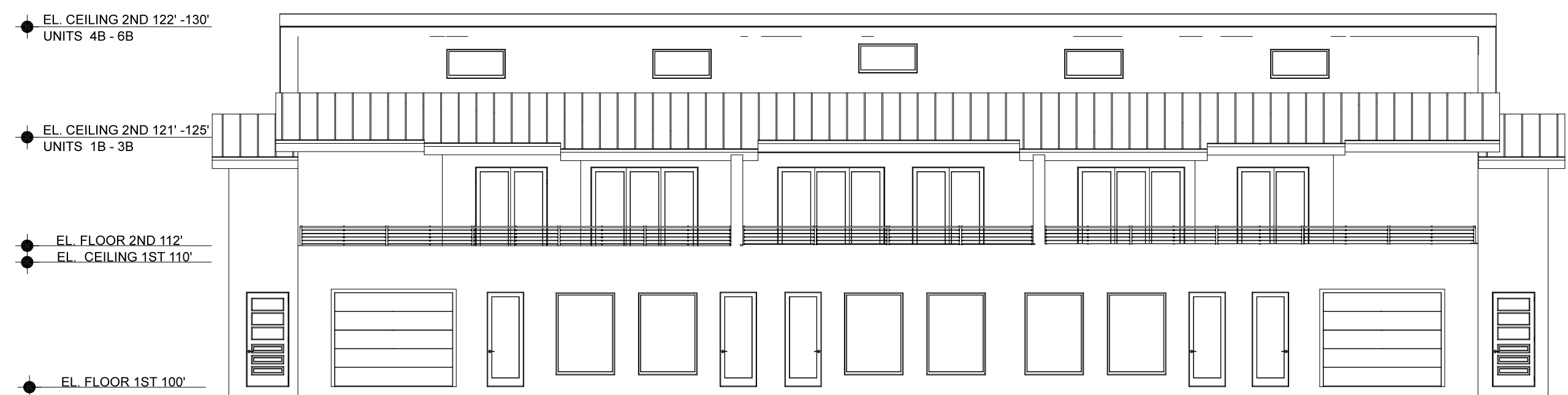
FRONT BUILDING
