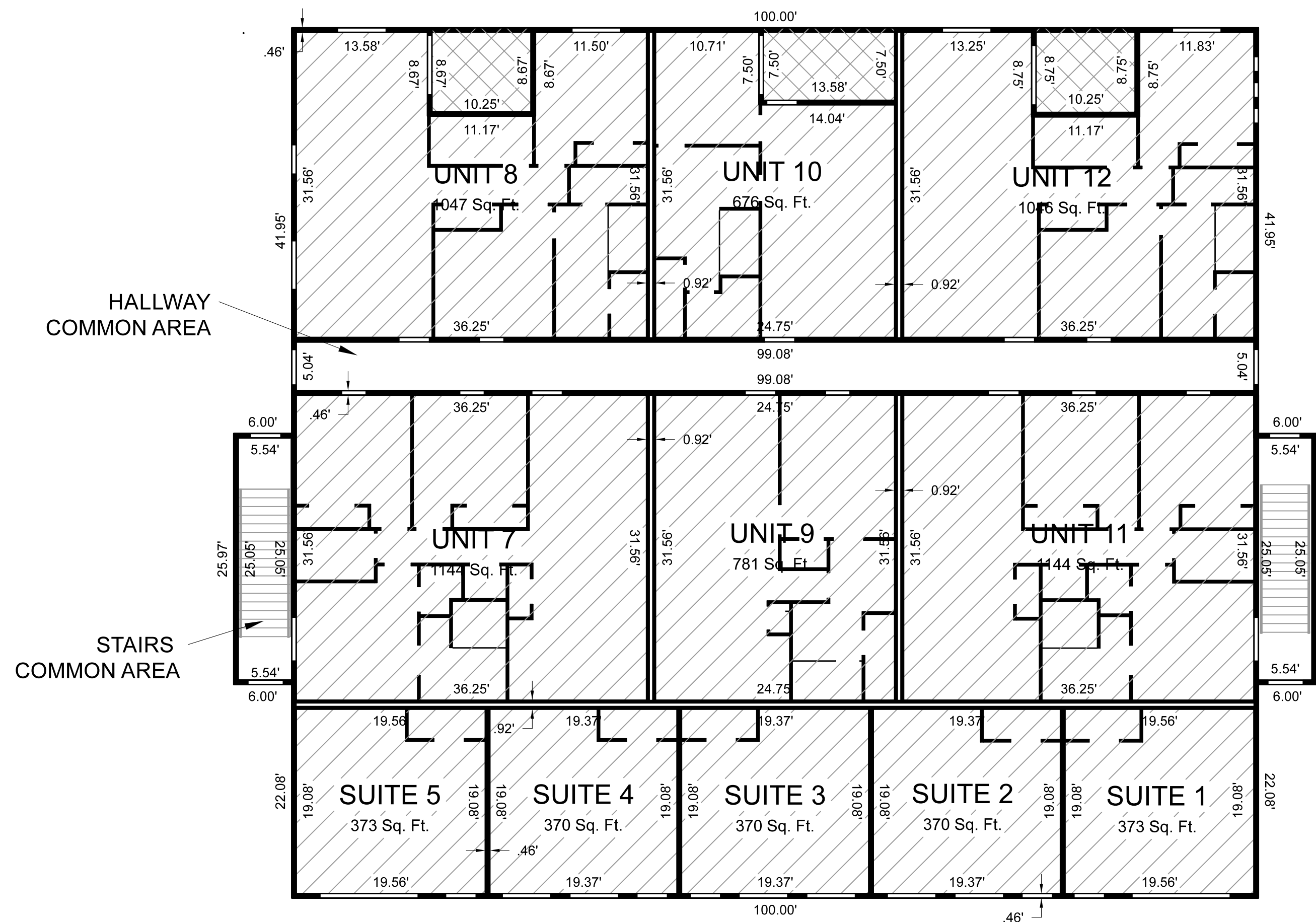
FIRST FLOOR
