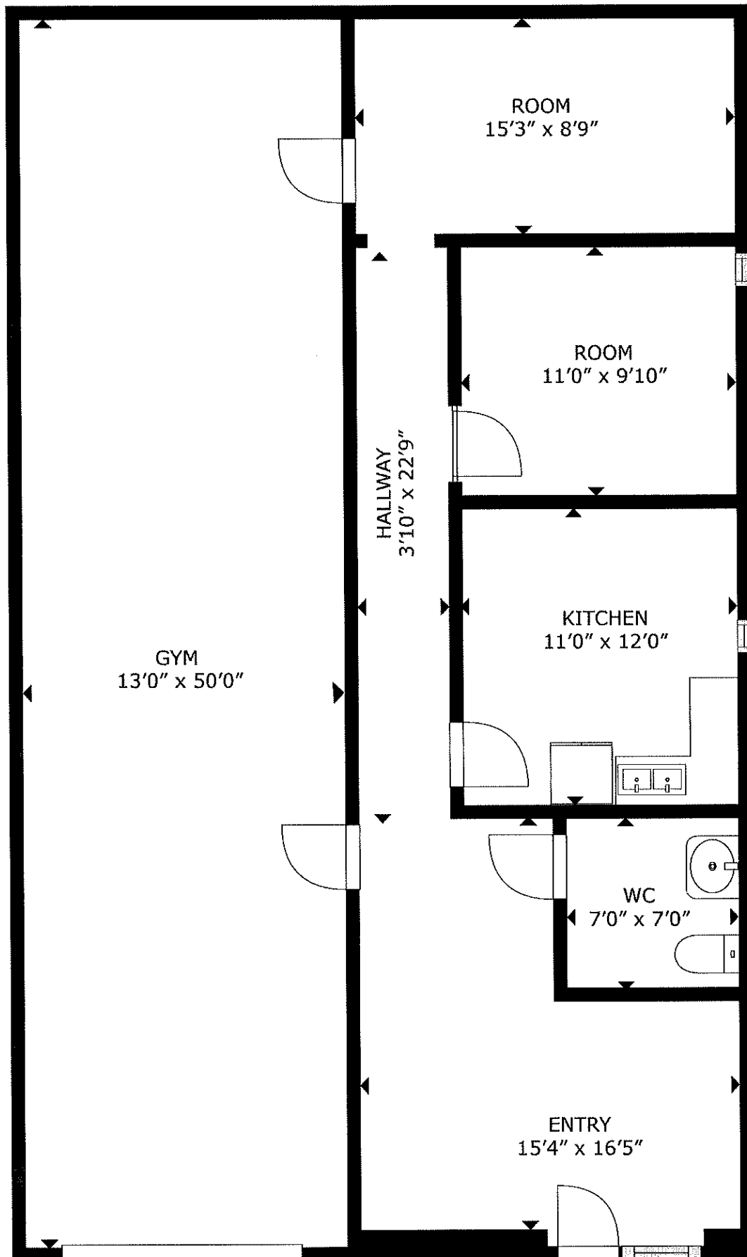
FLOOR PLAN
