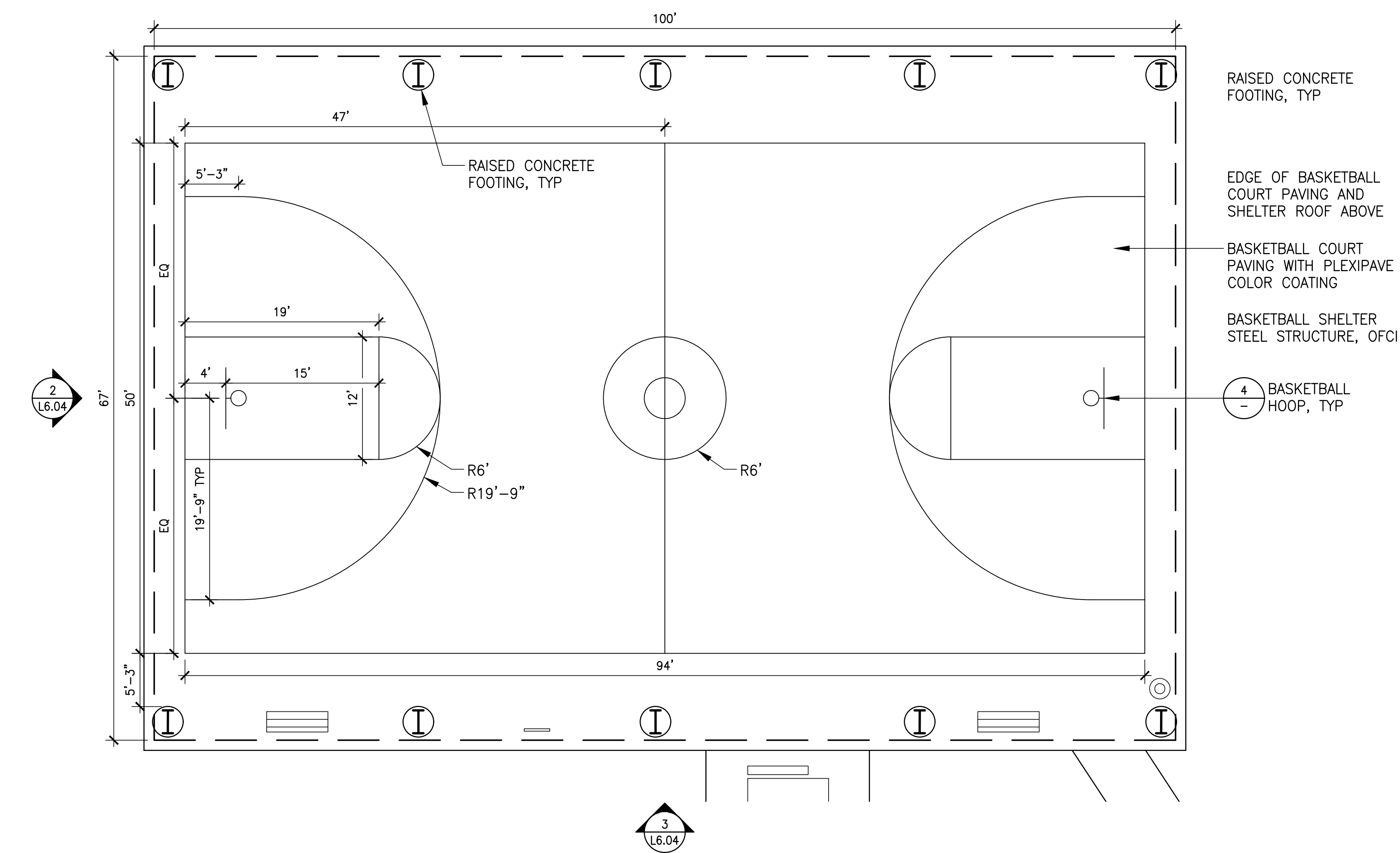
1 BASKETBALL COURT PLAN ENLARGEMENT
