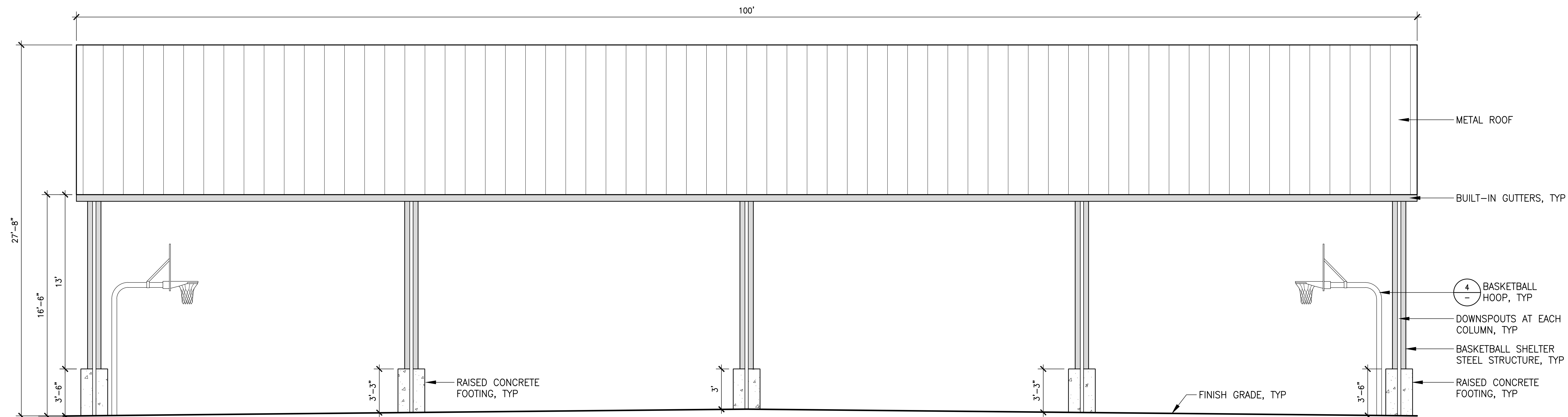
3 BASKETBALL COURT SHELTER SIDE ELEVATION
