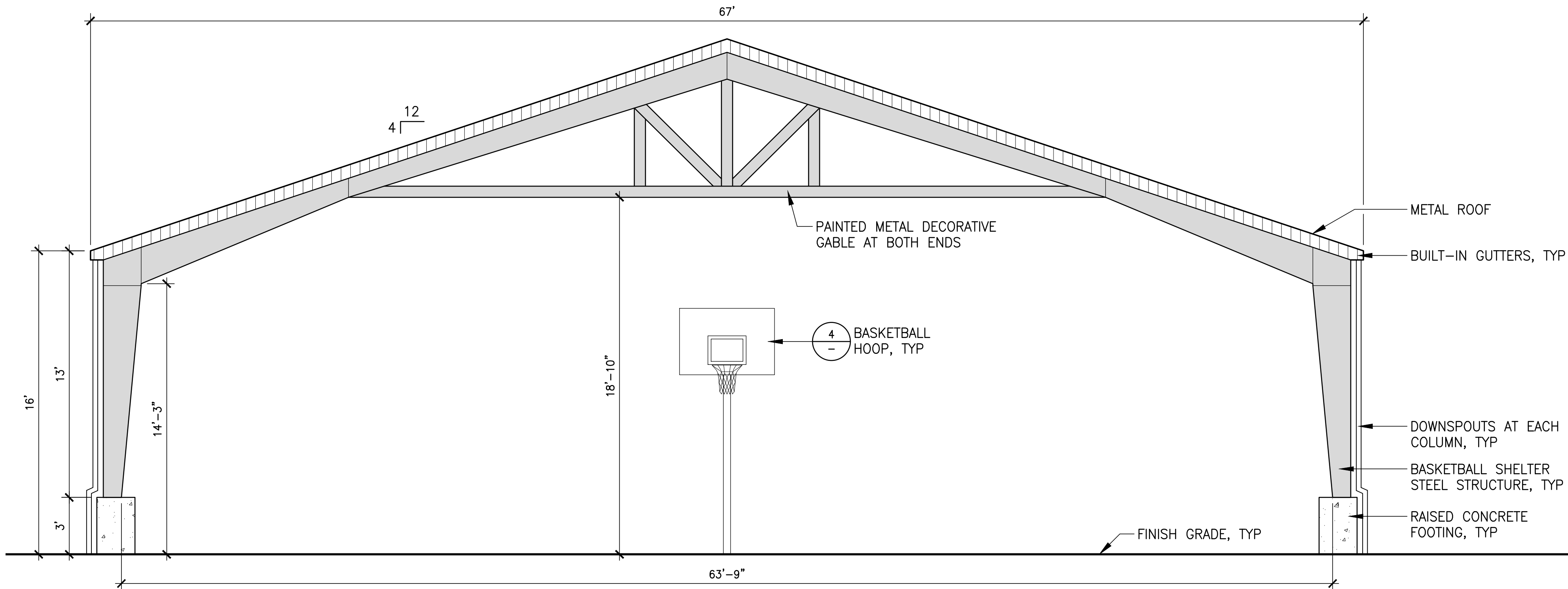
2 BASKETBALL COURT SHELTER END ELEVATION
