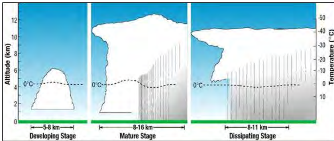
Figure 4-22 Thunderstorm Life Cycle
