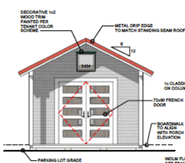
6 FRONT ELEVATION 1/8" = 1'-0"
