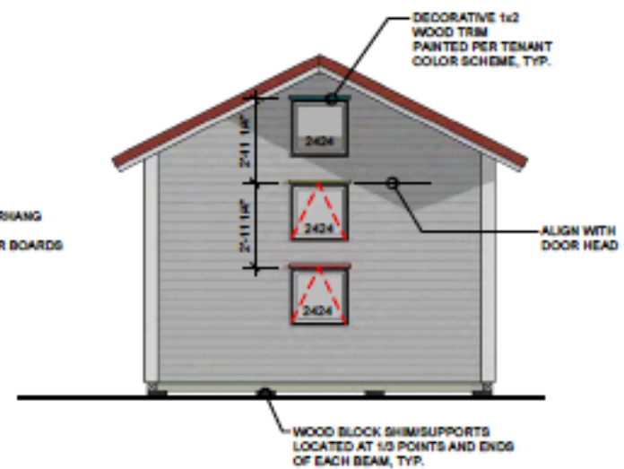
8 REAR ELEVATION 1/8" = 1'-0"
