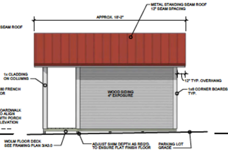
7 SIDE ELEVATION (TYP. BOTH SIDES EXCEPT FOR A.C. UNIT) 1/8" = 1'-0"
