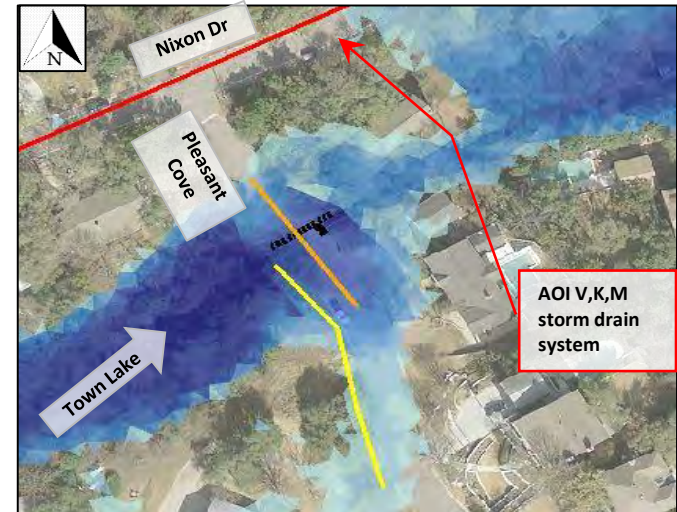
Proposed road improvements in orange, channel improvements in yellow. Existing culverts in black. Existing 100-yr inundation shown.
