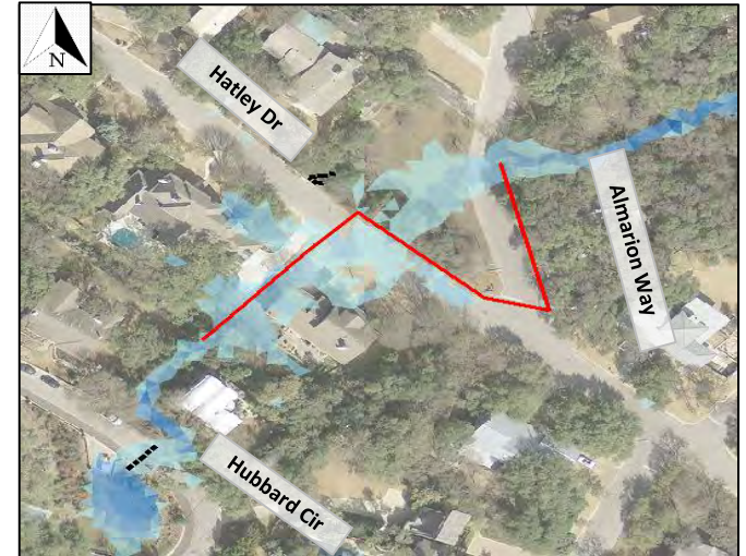
Proposed storm sewer in red. Existing 100-yr inundation shown.
