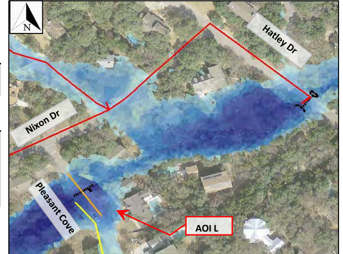
Proposed storm sewer in red. Proposed 12" curb in blue. Existing culvert in black. Existing 100-yr inundation shown.
