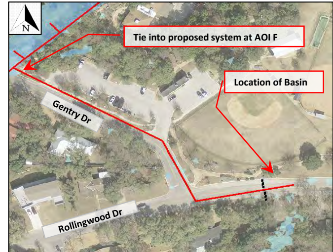
Rollingwood Drive, proposed storm sewer in red. Existing 100-yr inundation shown.
