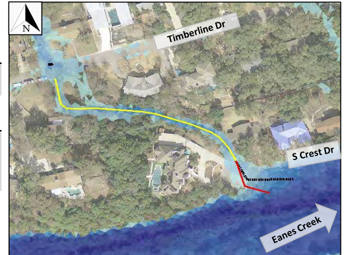
Channel improvements in yellow, proposed storm sewer in red. Existing channel in black. Existing 100-yr inundation shown.
