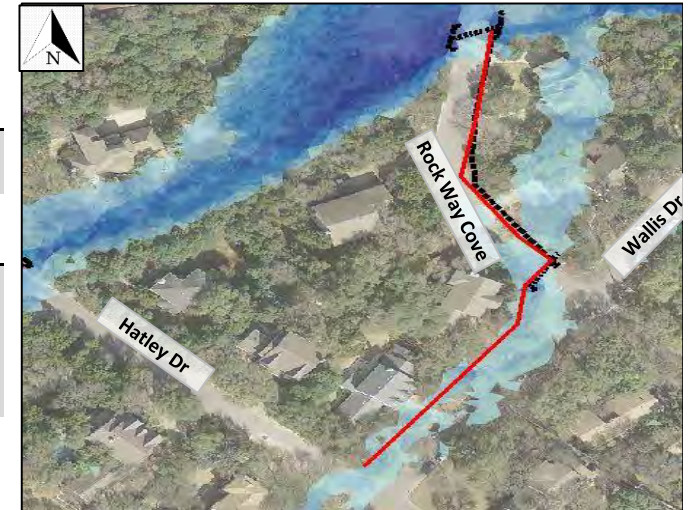
Proposed storm sewer in red, existing in black. Existing culverts in black. Existing 100-yr inundation shown.
