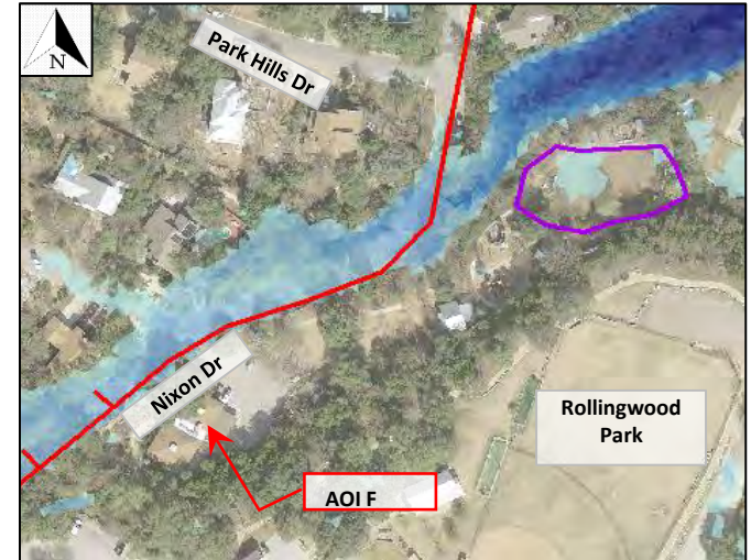
Proposed storm sewer (AOI F) and pond area in purple. Existing 100-yr inundation shown.
