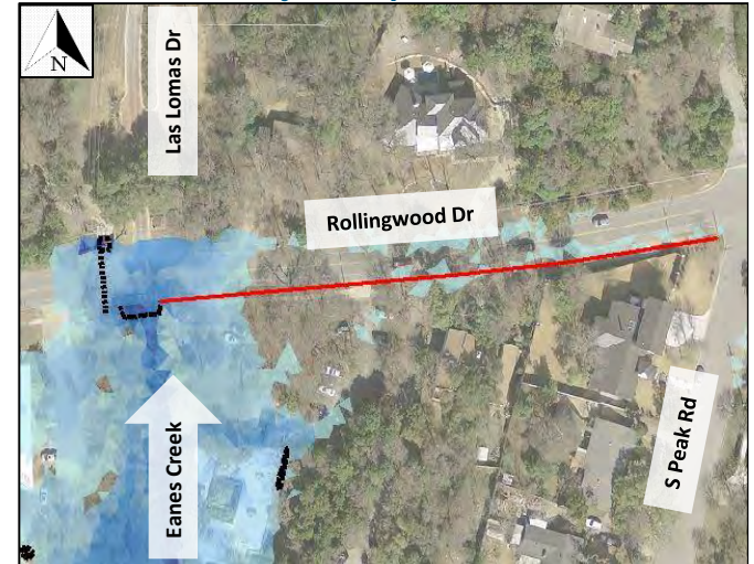
Proposed storm sewer in red. Existing culverts in black. Existing 100-yr inundation shown.
