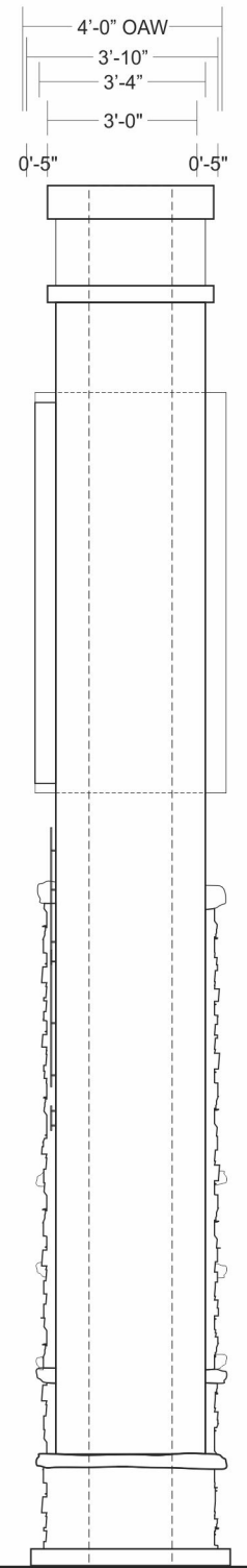
NORTH ELEVATION RIGHT SIDE
