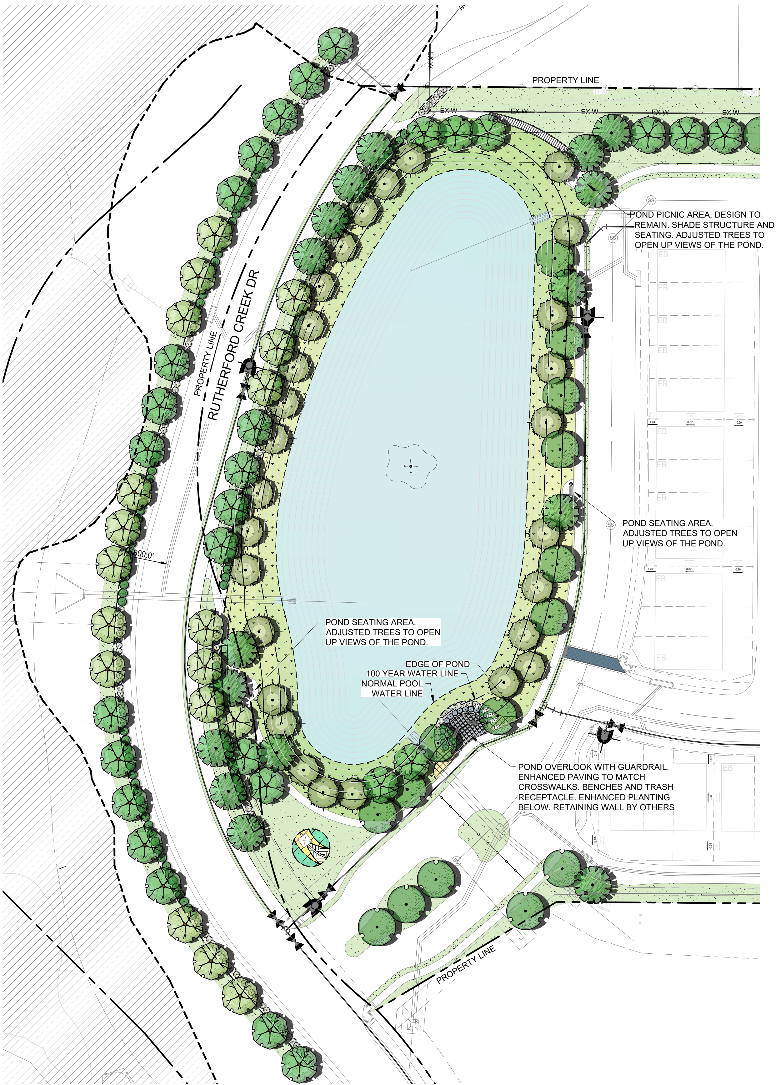
1 POND AMENITIES EXHIBIT 1" = 40'-0"
