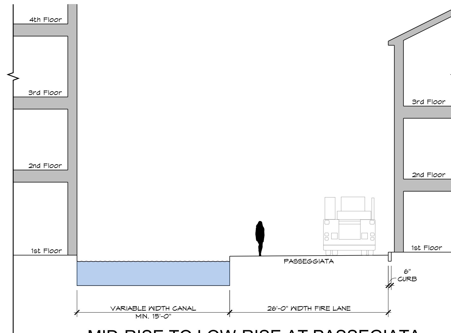
MID-RISE TO LOW-RISE AT PASSEGIATA
