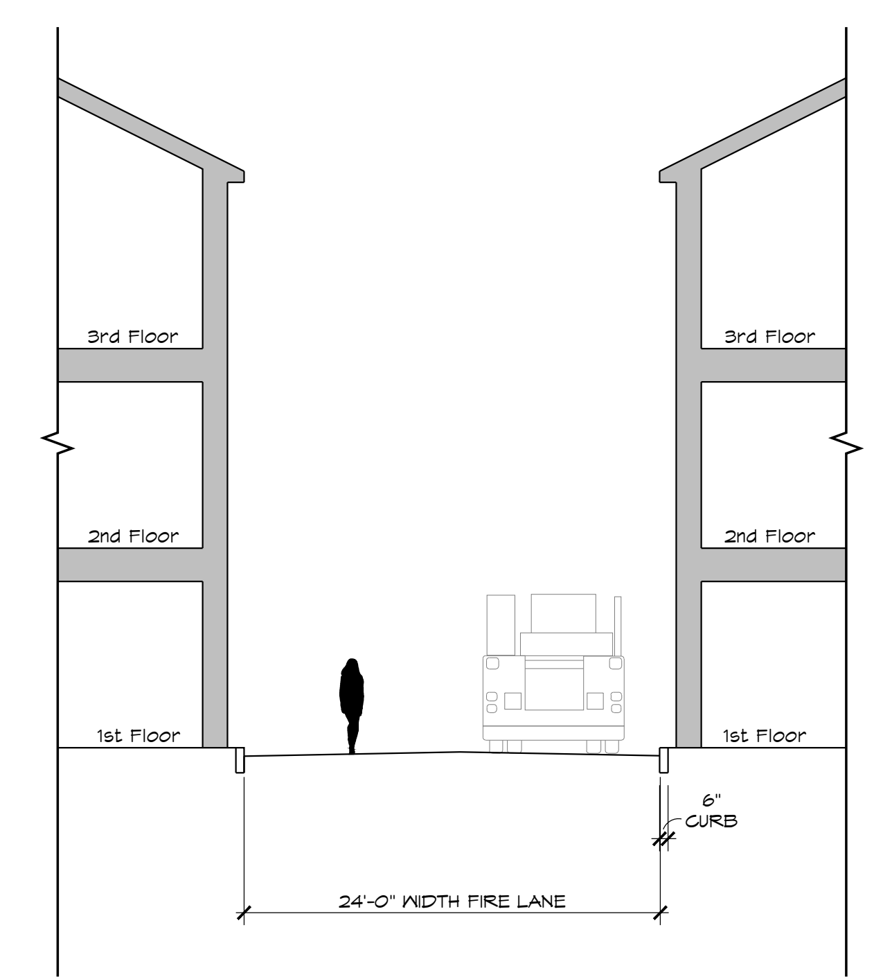
LOW-RISE TO LOW-RISE CORRIDOR
