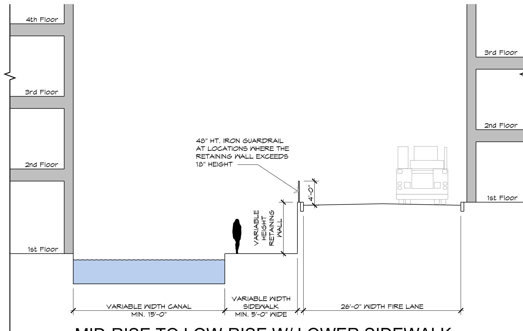
MID-RISE TO LOW-RISE W/ LOWER SIDEWALK
