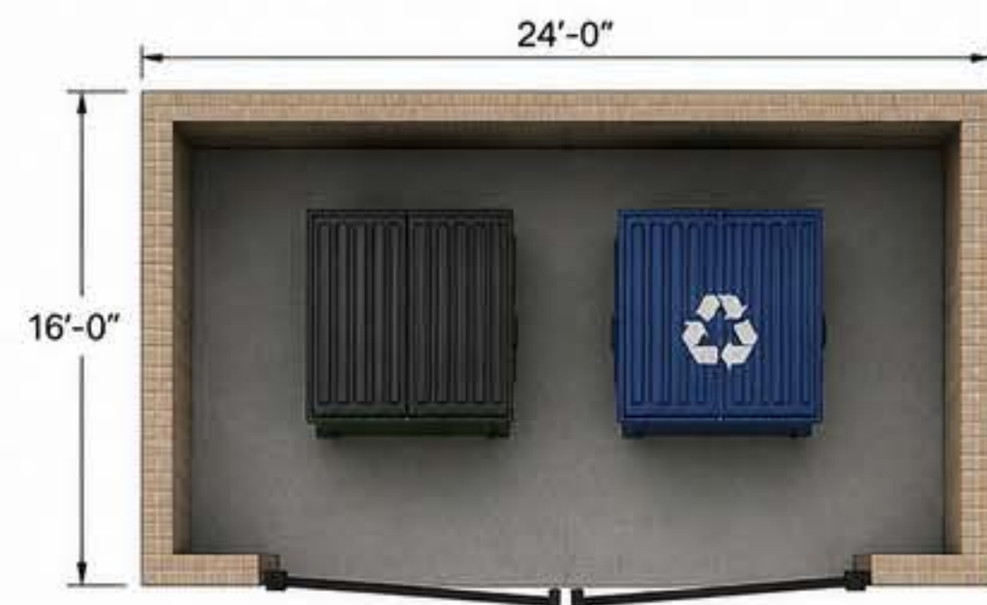
PLAN VIEW (24'-0" WIDE x 16'-0" DEEP)
