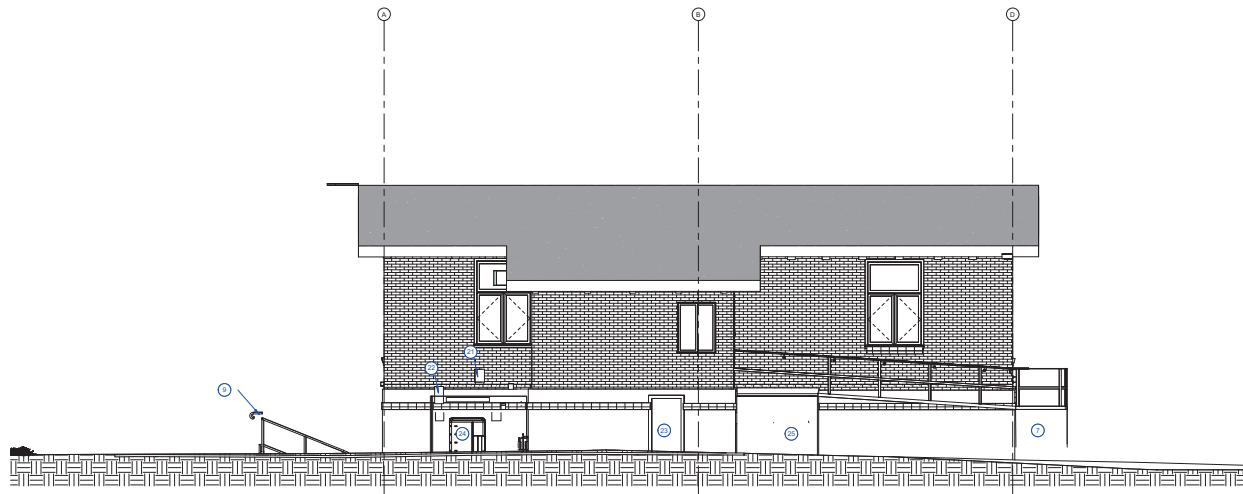
2 WEST ELEVATION 1/4" = 1'-0"
