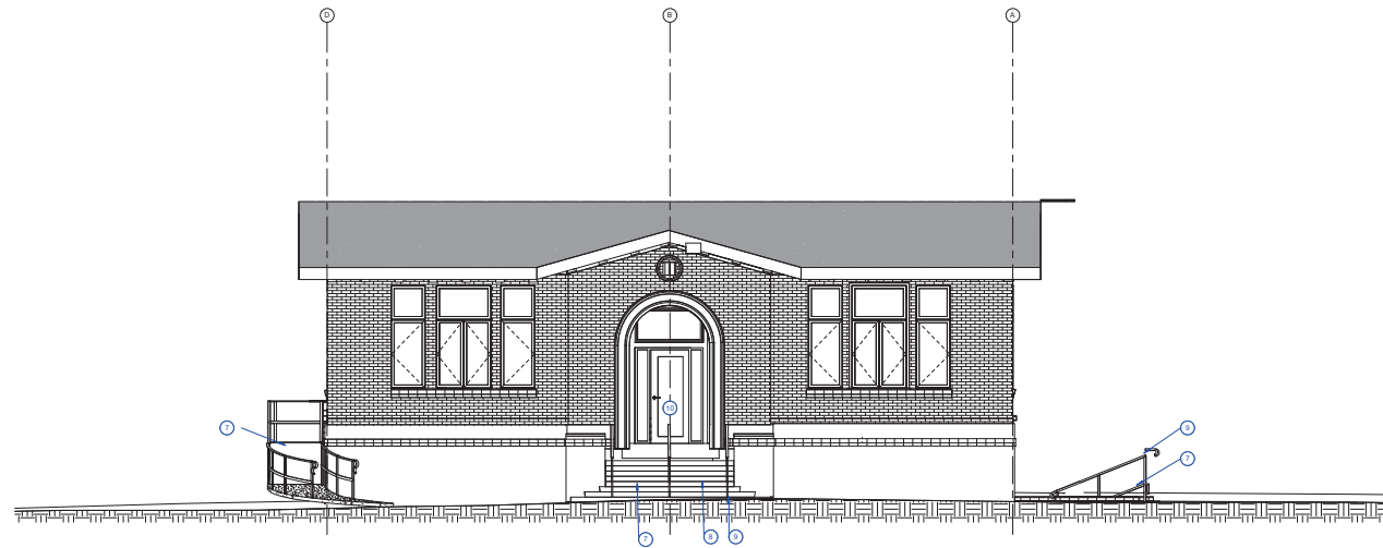
2 EAST ELEVATION 1/4" = 1'-0"
