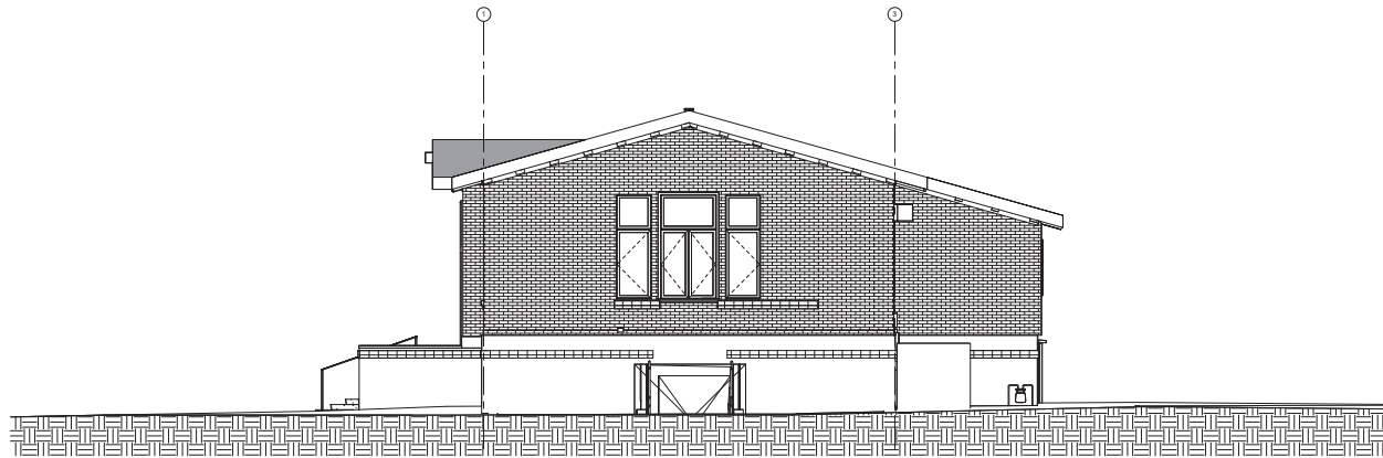
1 NORTH ELEVATION 1/4" = 1'-0"
