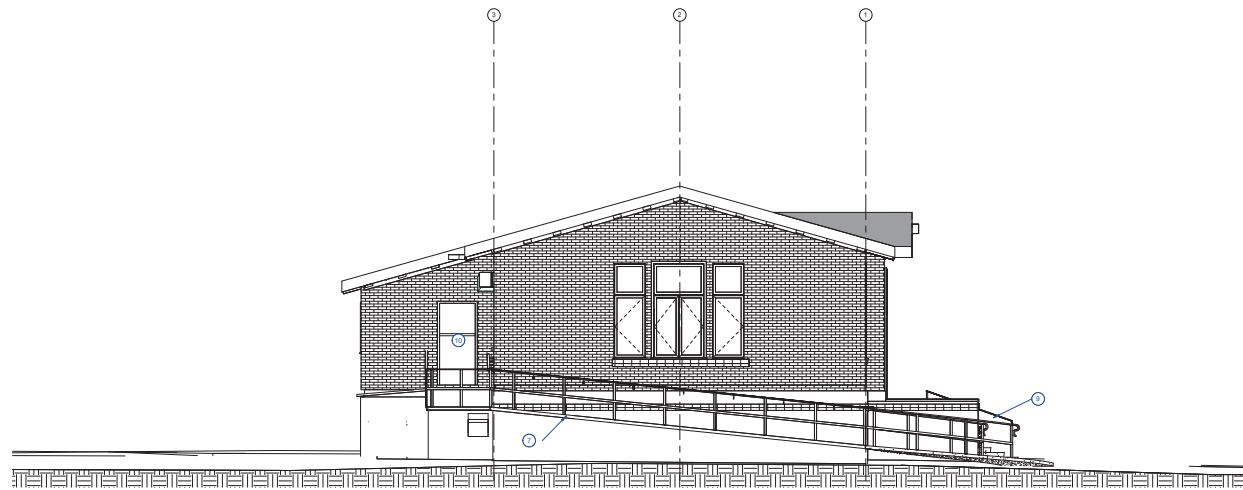
1 SOUTH ELEVATION 1/4" = 1'-0"
