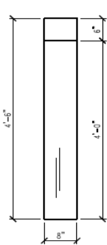
END VIEW
