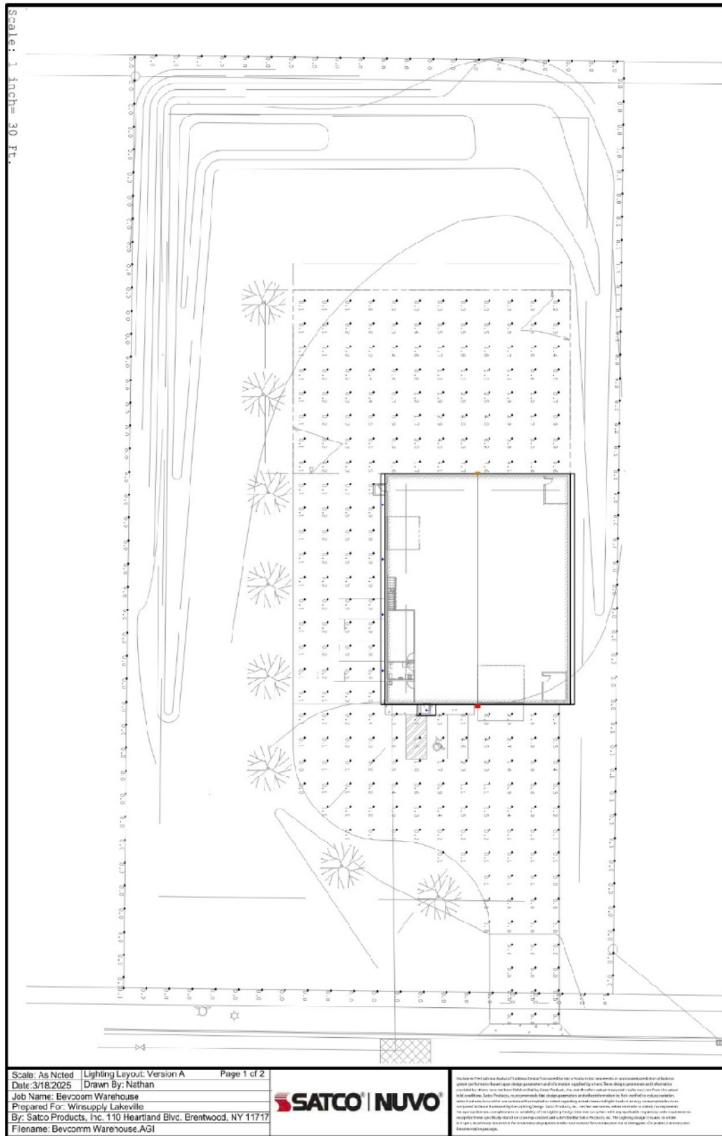
Photometric Plan
