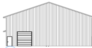
2 WEST ELEVATION SCALE: 1/16" = 1'-0"
