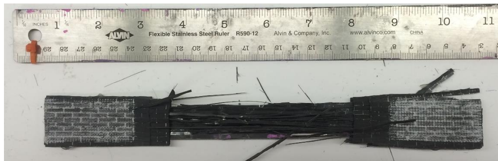
Figure 1.2 – Representative failure mode MGM: Multiple (Longitudinal Splitting and Lateral), at Gage, in the Midele
