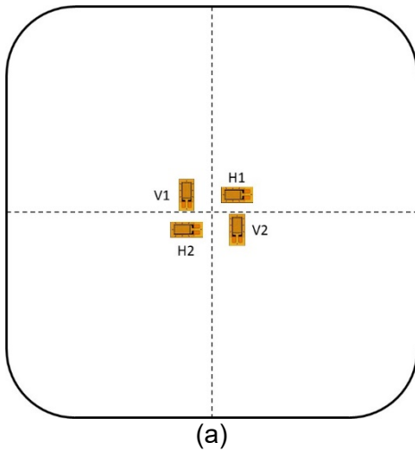
Figure 3 – Additional instrumentation (strain gages) used for Specimens 130F-3 and 130F-4
