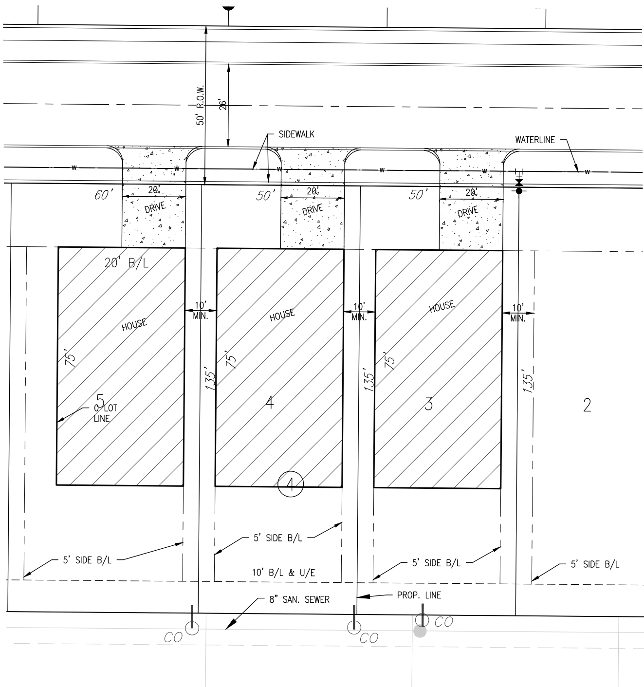
EXHIBIT "A" TYPICAL LOT PLAN HALLBROOKE ADDITION PLANNED UNIT DEVELOPMENT NOT TO SCALE
