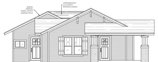
1 PROPOSED FRONT ELEVATION SCALE: 1/4" = 1'-0"
