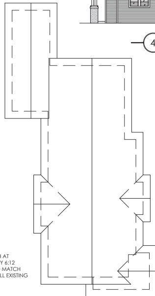
5 EXISTING ROOF PLAN SCALE: 1/8" = 1'-0"
