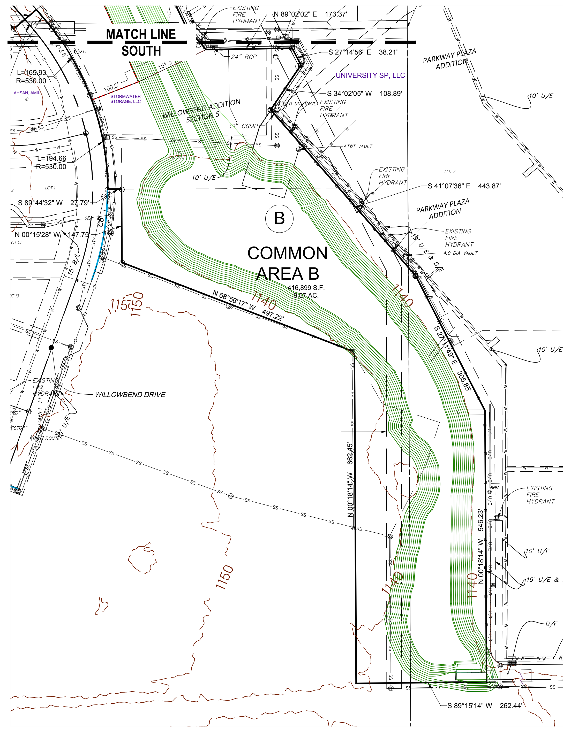
SOUTH AREA
