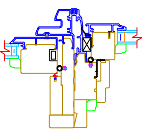
USA ARCHITECTURAL DOUBLE HUNG 0" Mull Shown w/ OPTIONAL 1", 1 1/2", 2", 3", OR 4"
