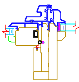
USA ARCHITECTURAL DOUBLE HUNG 0" Mull Shown w/ OPTIONAL 1", 1 1/2", 2", 3" OR 4"
