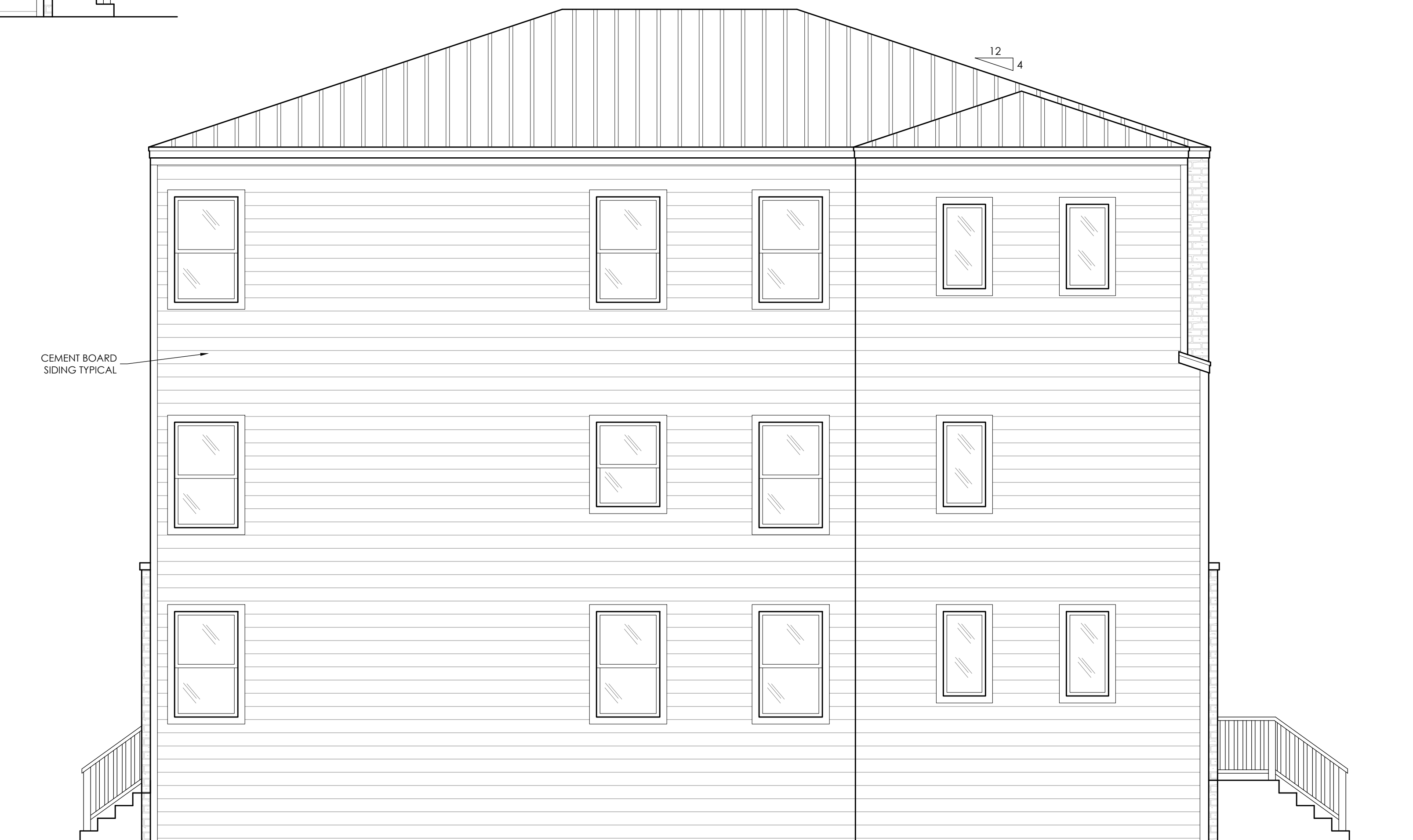
LEFT ELEVATION 1/4"=1'-0"
