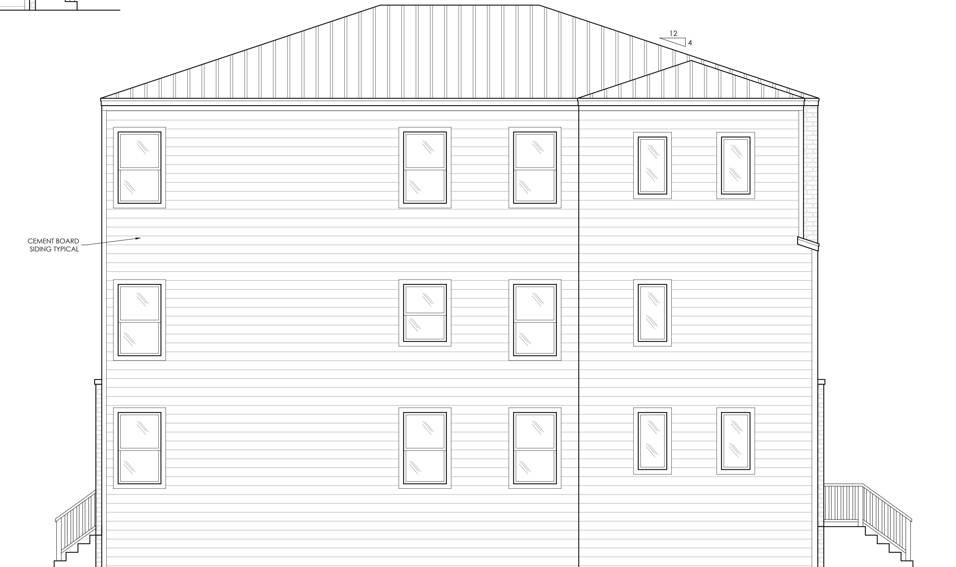
LEFT ELEVATION 1/4"=1'-0"
