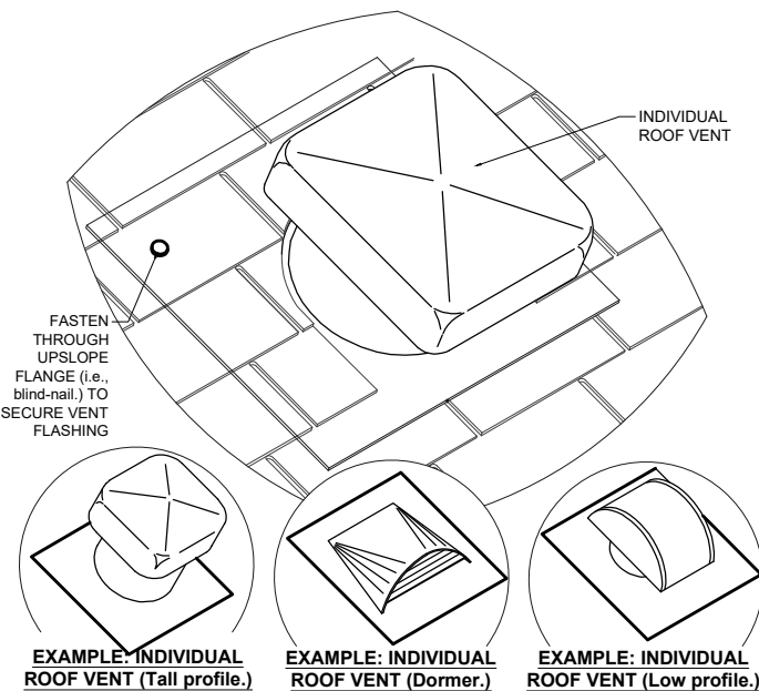
B ROOF VENT DETAIL NTS
