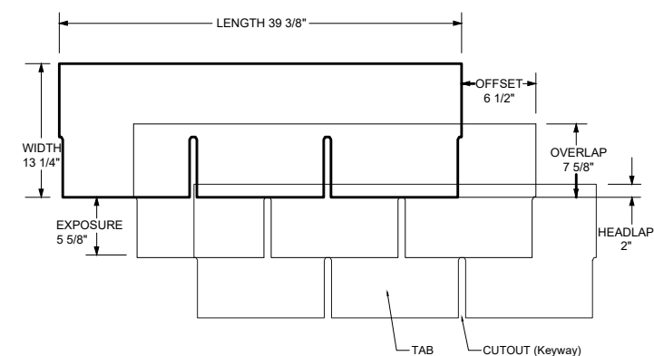
C BASIC SHINGLE COURSE - LAMINATED NTS
