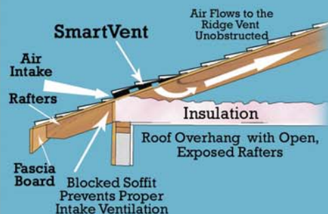
Mid-Roof Intake
