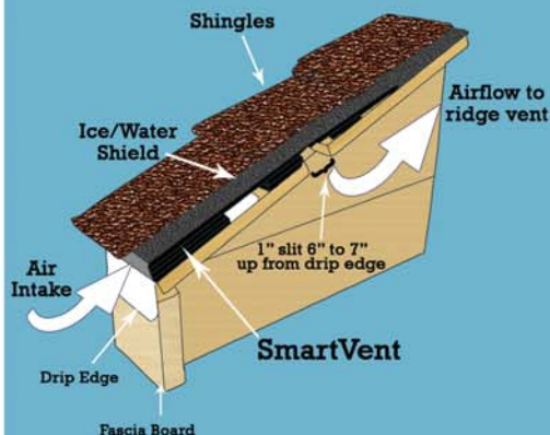
Eave Intake
