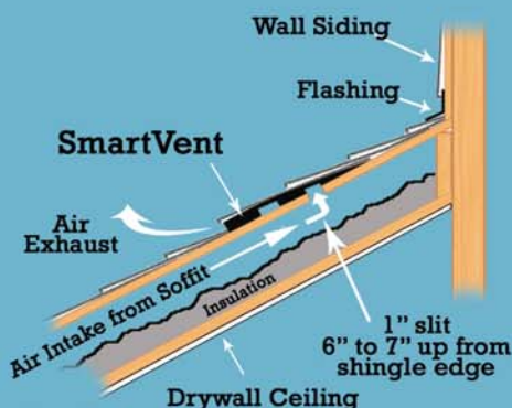
Off-Wall Shed Roof Exhaust
