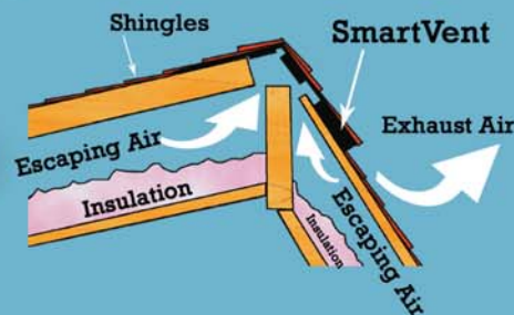
Dormer Peak Exhaust
