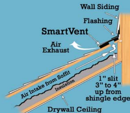
Shed Wall Flash Exhaust
