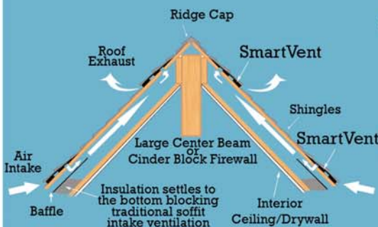
Off-Peak / Firewall Exhaust
