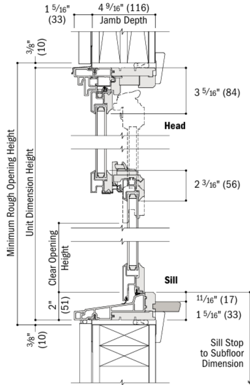
Vertical Section
