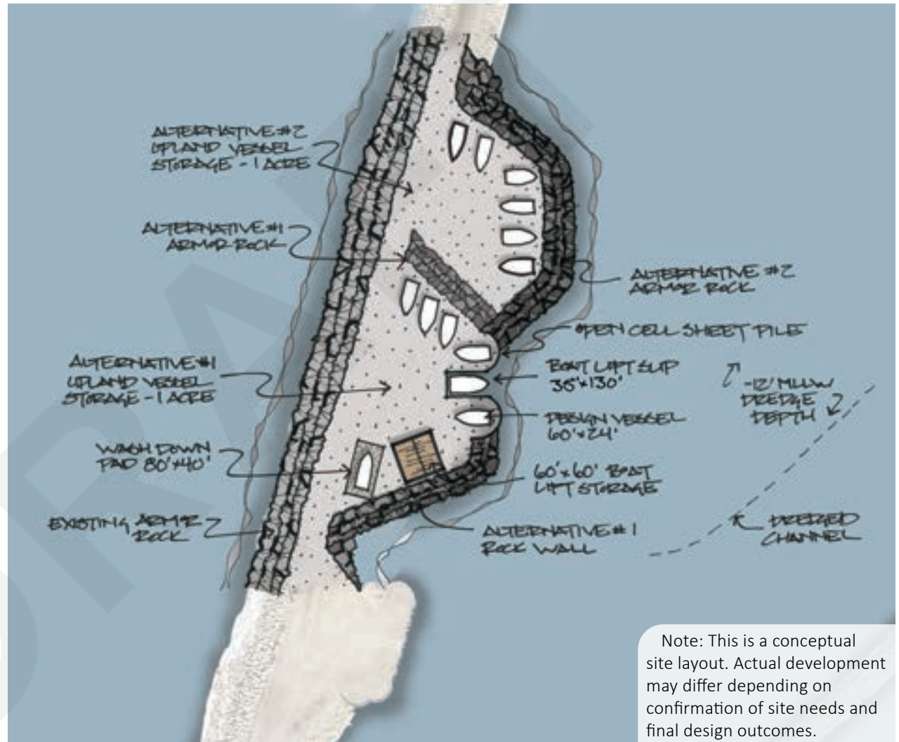
Travel Lift - Option 2
