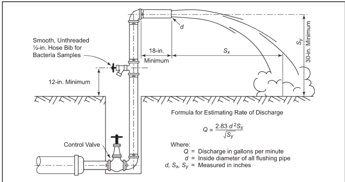
Figure 2: Combination blowoff and sampling tap
