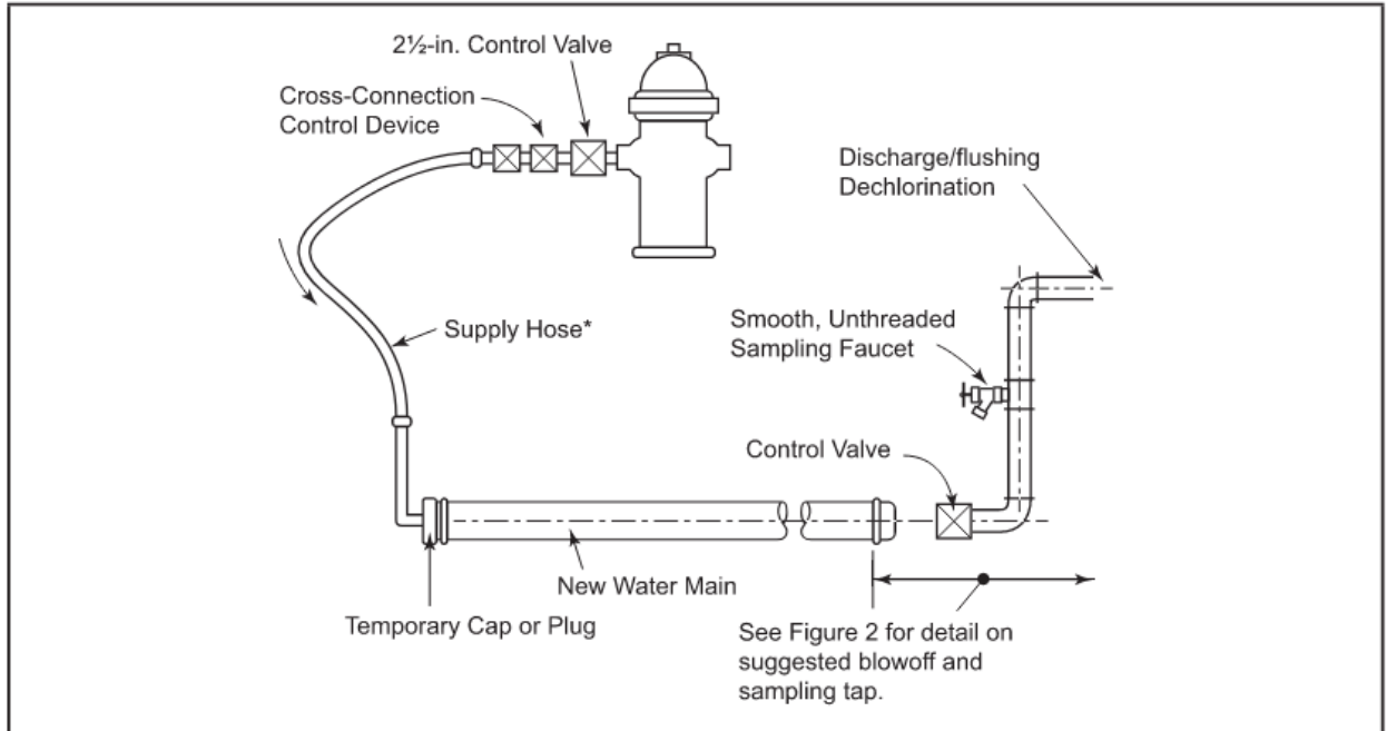
Figure 1: Temporary flushing/testing connection
