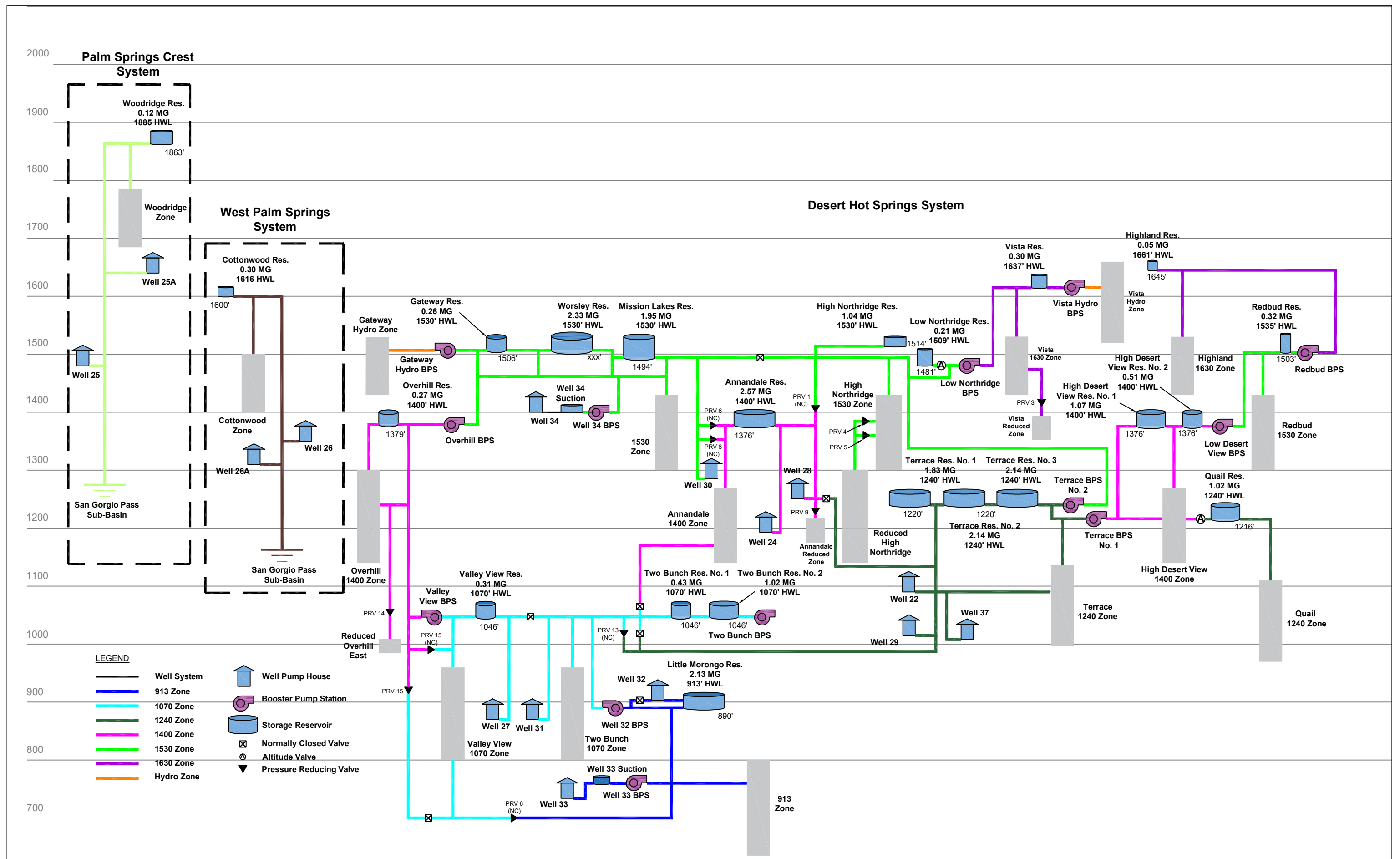
Figure 2.3 Existing System Hydraulic Schematic
