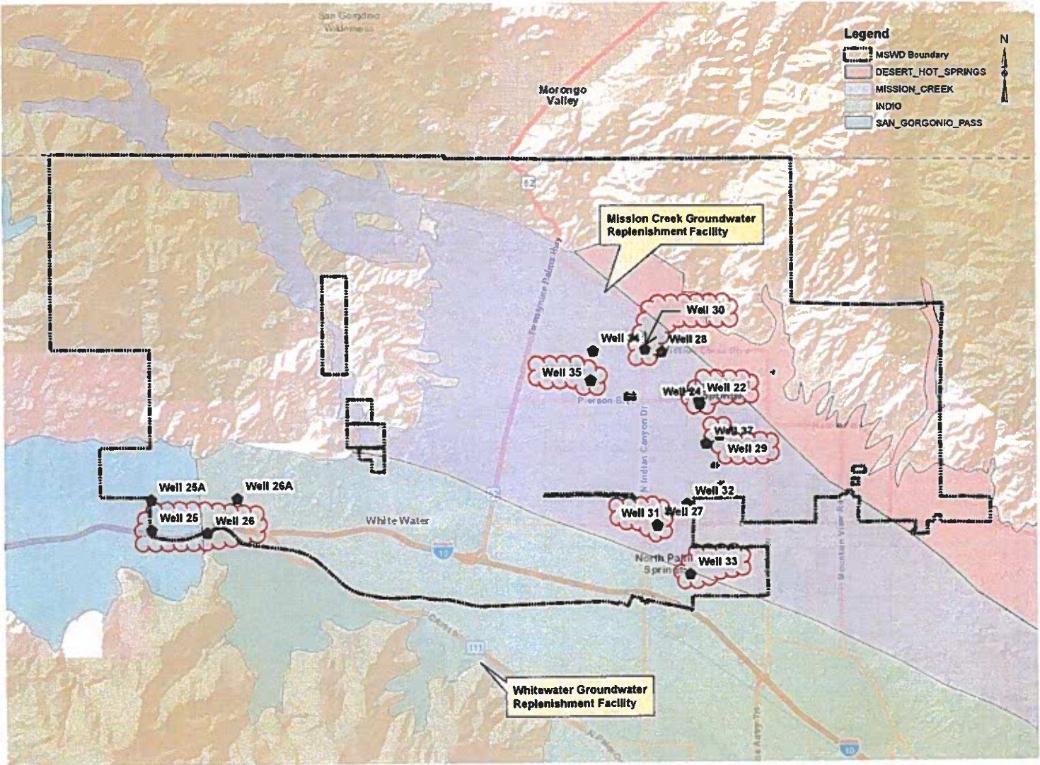
Figure 3.1 - Groundwater Subbasins
