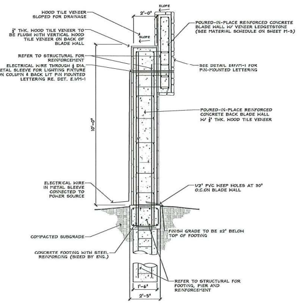
(C) SECTION 'B-B' Scale: NTS
