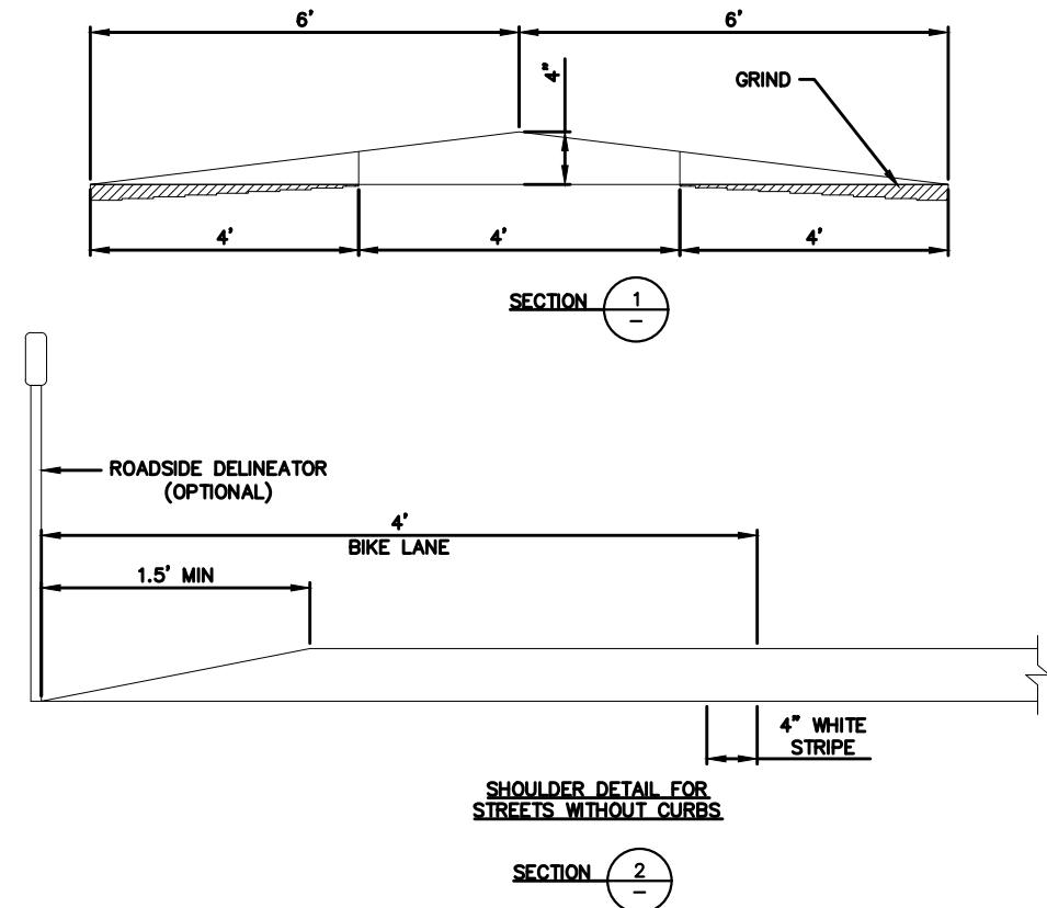
SPEED HUMP SECTION DETAIL
