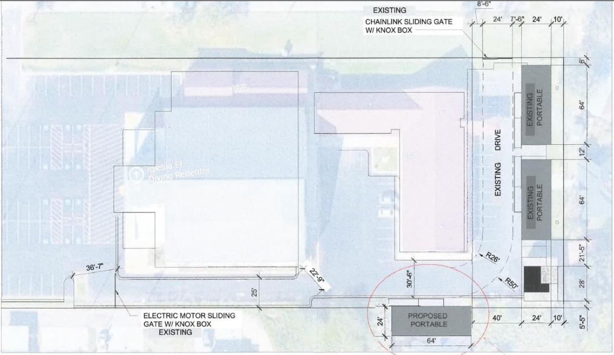
01 PROPOSED PORTABLES OPTION 1
