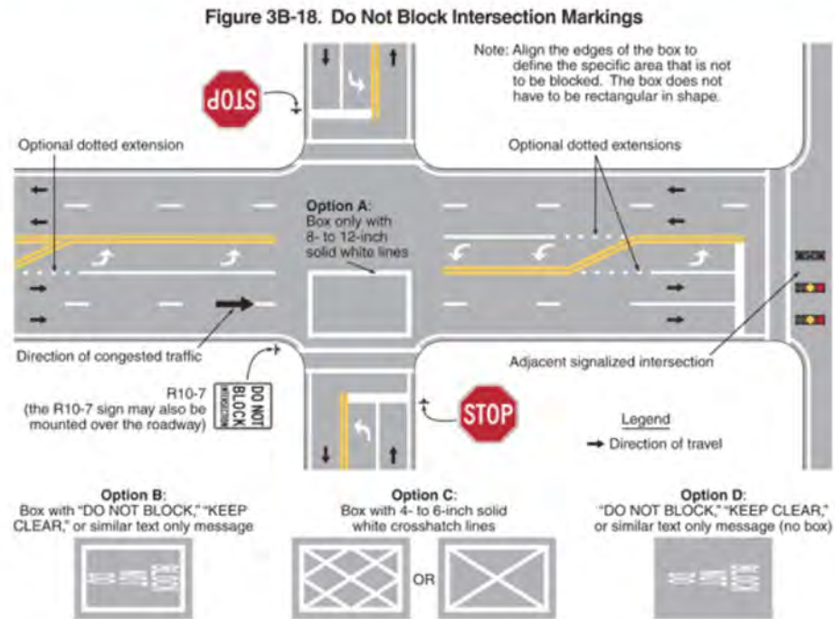
Figure 3B-18. Do Not Block Intersection Markings
