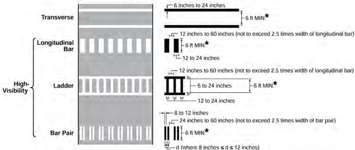
Figure 3C-1. Crosswalk Markings
