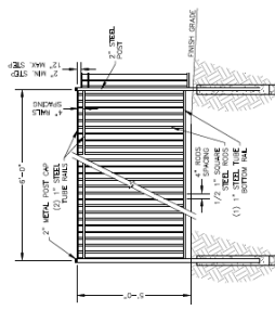
01 6' HEIGHT OPEN VISION METAL FENCE
