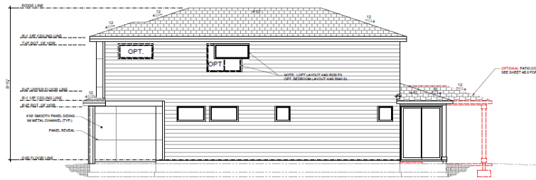
RIGHT ELEVATION "G" (SLEEK CONTEMPORARY)
