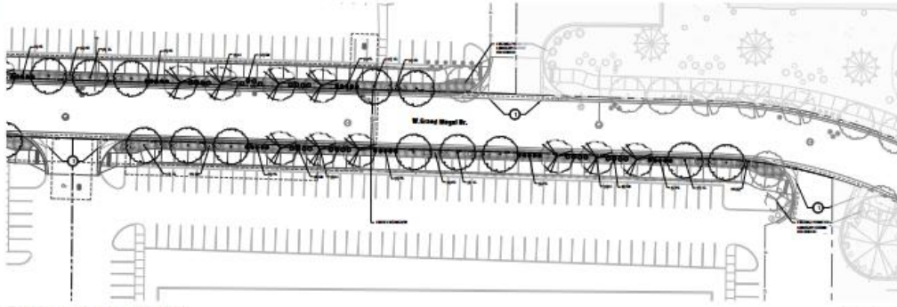
Landscape - Grand Mogul East Area
