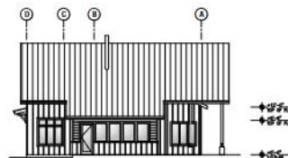
2 SIDE ELEVATION (EAST) Scale: 1/4" = 1'-0"
