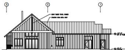
3 REAR ELEVATION (NORTH) Scale: 1/4" = 1'-0"
