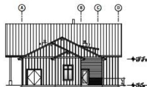
4 SIDE ELEVATION (WEST) Scale: 1/4" = 1'-0"
