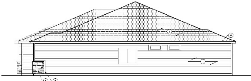
3B SIDE ELEVATION TYP. - HIP ROOF OPTION
