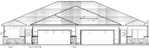
1B ENTRY (FRONT) ELEVATION - HIP ROOF OPTION
