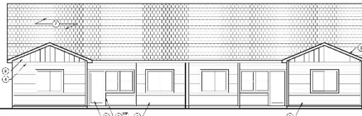
2A PATIO (REAR) ELEVATION - GABLE ROOF OPTION
