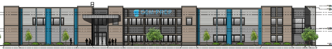
1 NORTH ELEVATION
