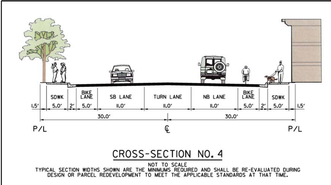
Figure 8. Cross-Section No. 4
