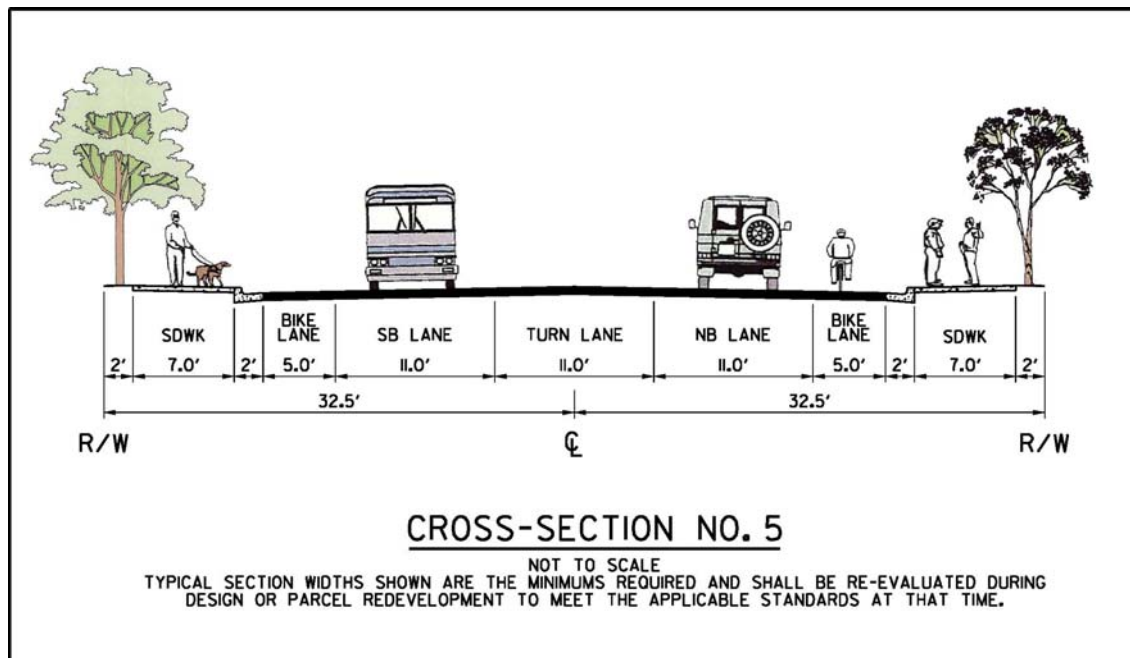
Figure 9. Cross-Section No. 5
