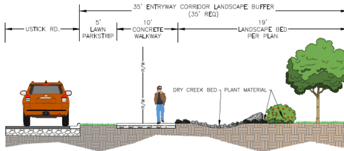
USTICK RD. LANDSCAPE BUFFER SECTION
