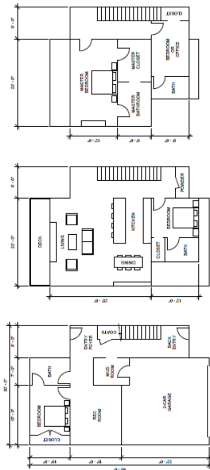
TYPICAL TOWNHOME 2,600sf LIVABLE + 470sf GARAGE
