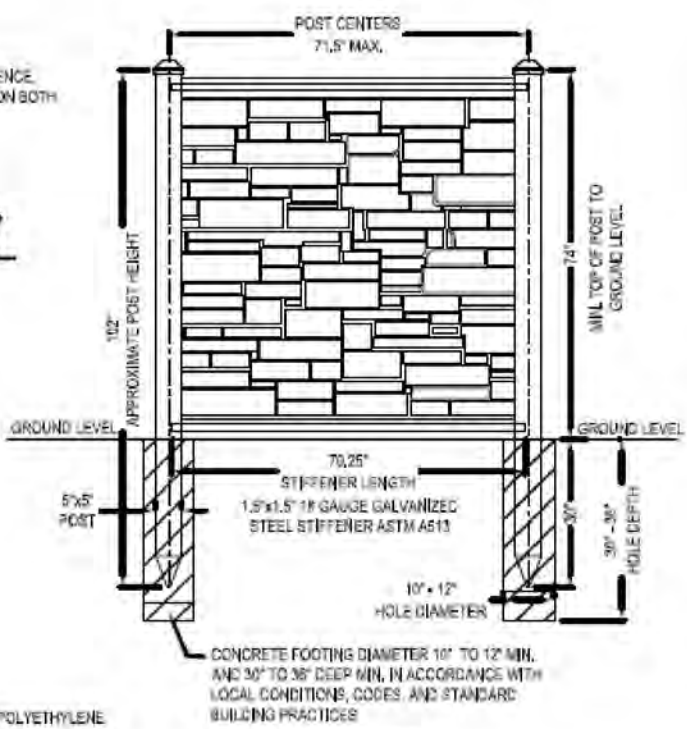
ELEVATION VIEW
