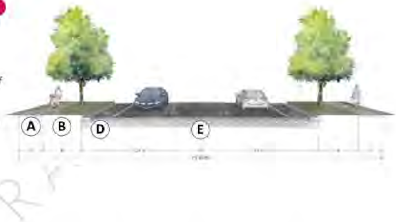
Figure 7.3 Typical Commercial Street Section, Two-Lane + Turn Lane + Bike Lanes
