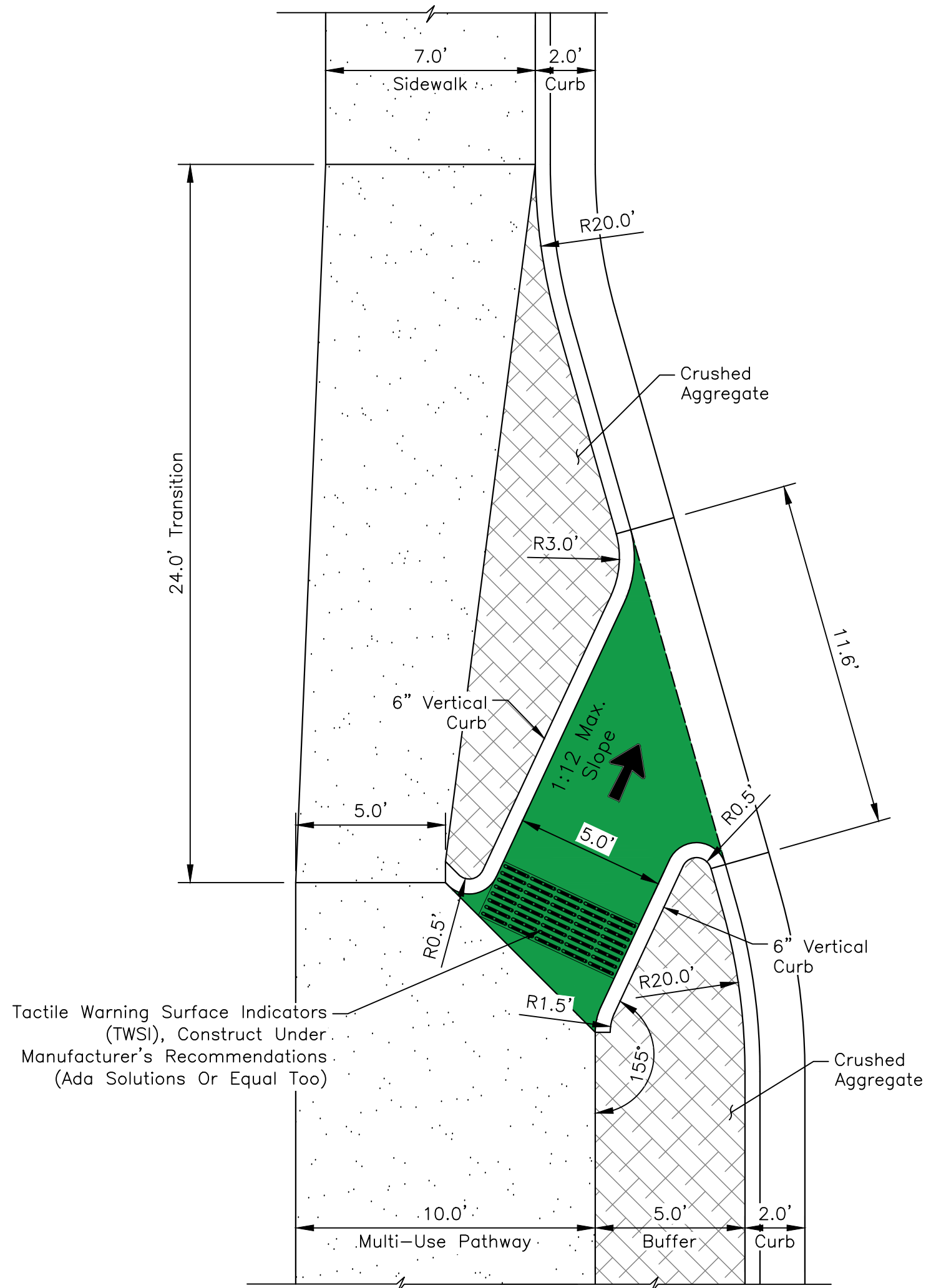
A1 BIKE RAMP - BIKE LANE/MULTI-USE PATH TRANSITION
