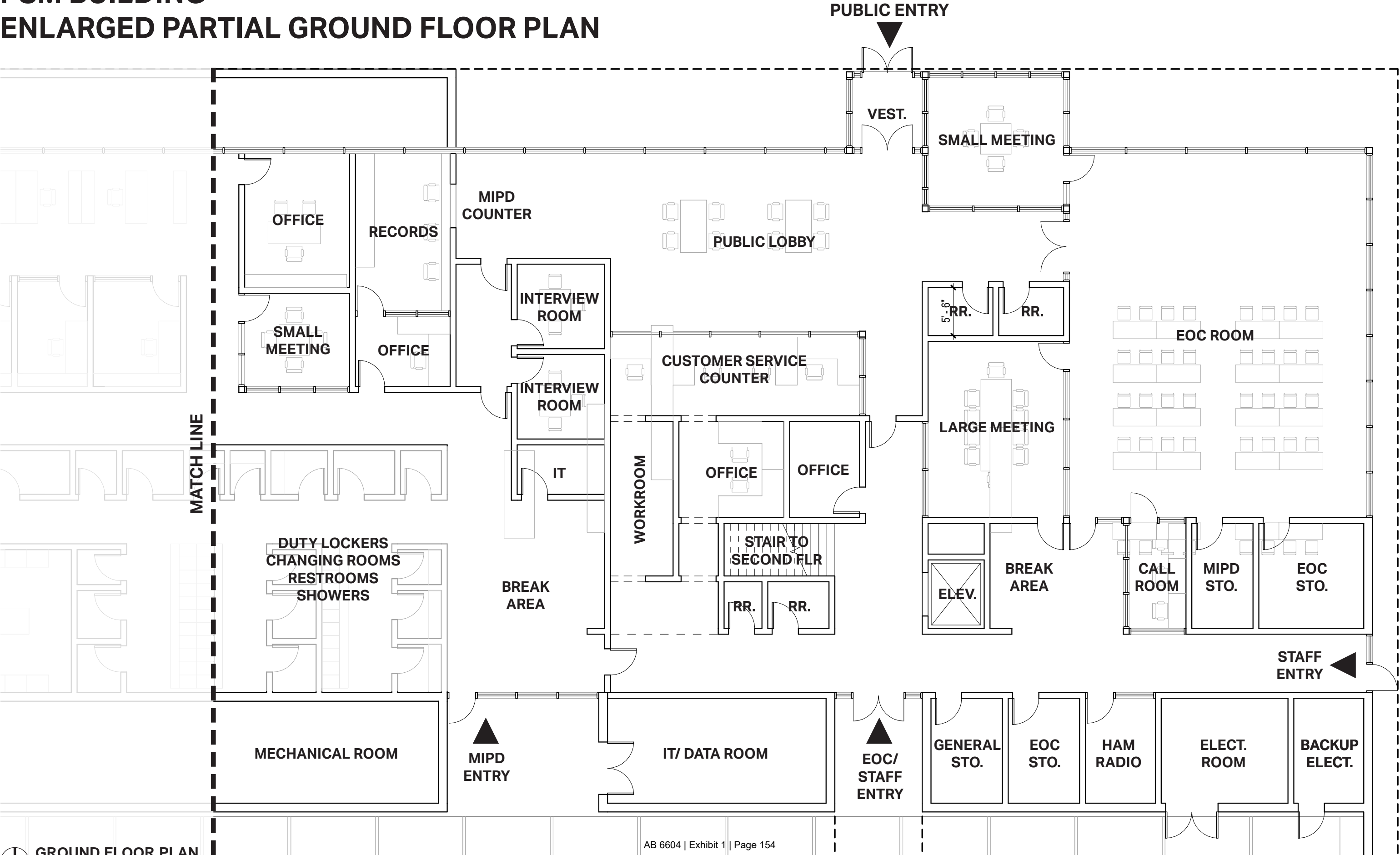
1 GROUND FLOOR PLAN 1" = 10'
