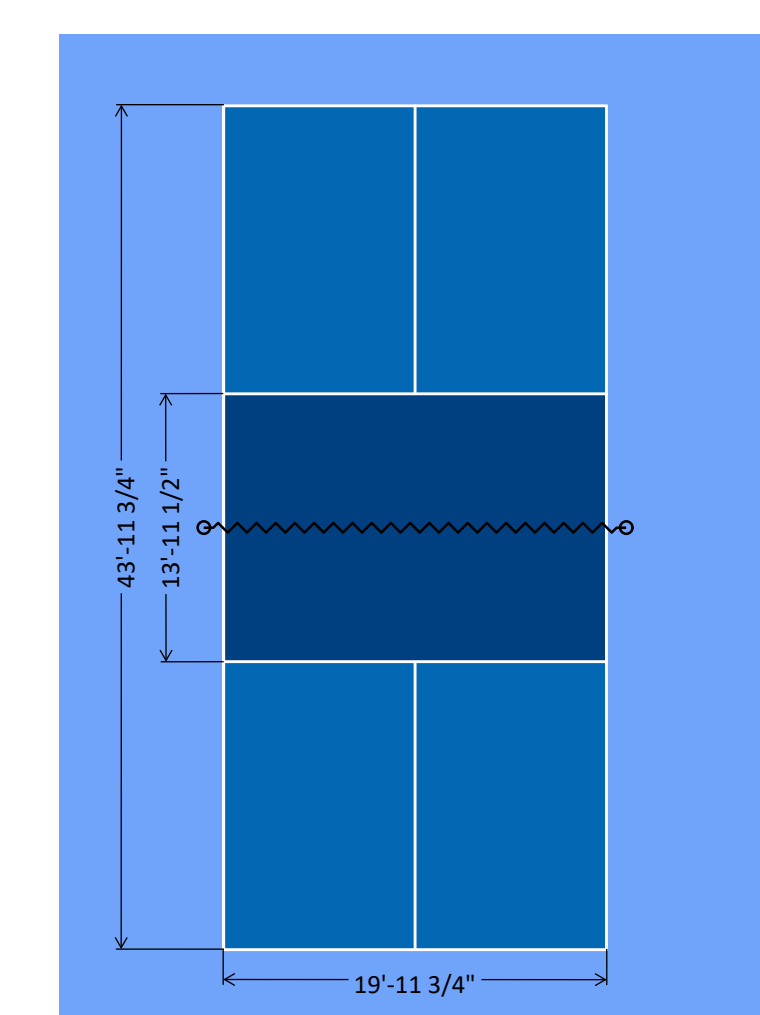
PICKLEBALL STANDARD LAYOUT Colors are approximate - manufacturers standard range may differ.
