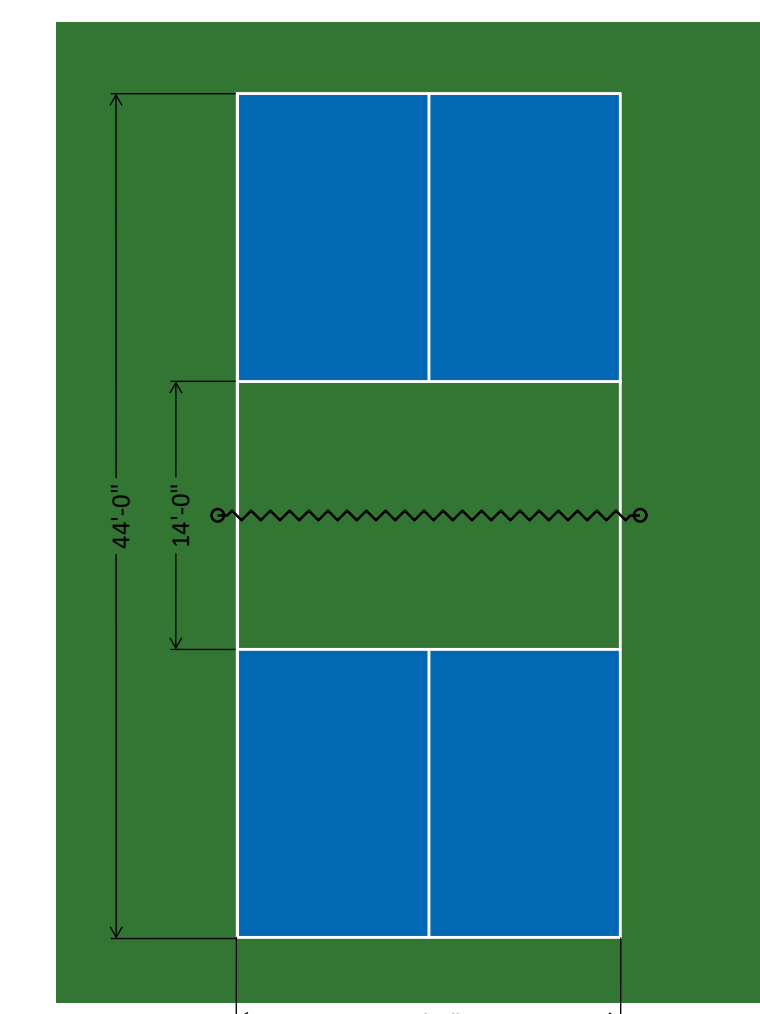
PICKLEBALL STANDARD LAYOUT Source: USA Pickleball 2023 (Color Scheme 1) Colors are approximate - manufacturers standard range may differ.
